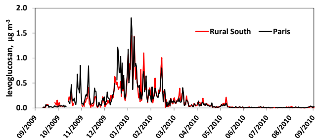
Figure 9. Daily levoglucosan values observed during the PARTICULES project from September 2009 to September 2010 at the downtown urban and southern rural sites. The rural site is located far from direct sources. Levoglucosan is a tracer for wood-burning emissions. The similar values at both sites ( R^2 = 0.83 , slope rural vs. downtown site 0.84) suggest a strong regional control of wood-burning-related organic aerosol.
