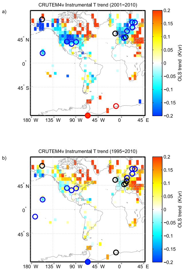
Figure S1: Same as Figures 5b and 6b , but for period of CRUTEM4v instrumental datasets. The temperature trends were calculated from variance adjusted monthly data of temperature anomalies, obtained from http://www.cru.uea.ac.uk/cru/data/temperature/
