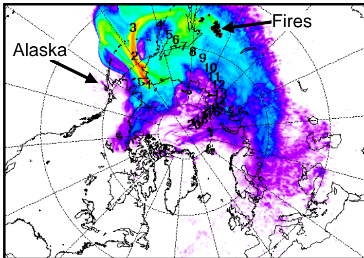
Polluted Case
