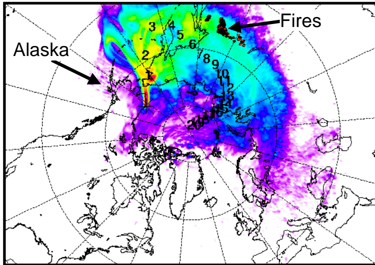
Warm-Polluted Case
