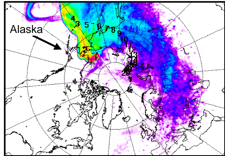
Clean Case
