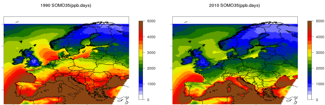
Figure 2.9: Modelled SOMO35 (ppb day) in the EURODELTA 6-model ensemble using 1990 (left) or 2010 (right) emissions and 2010 meteorological year and boundary conditions.
