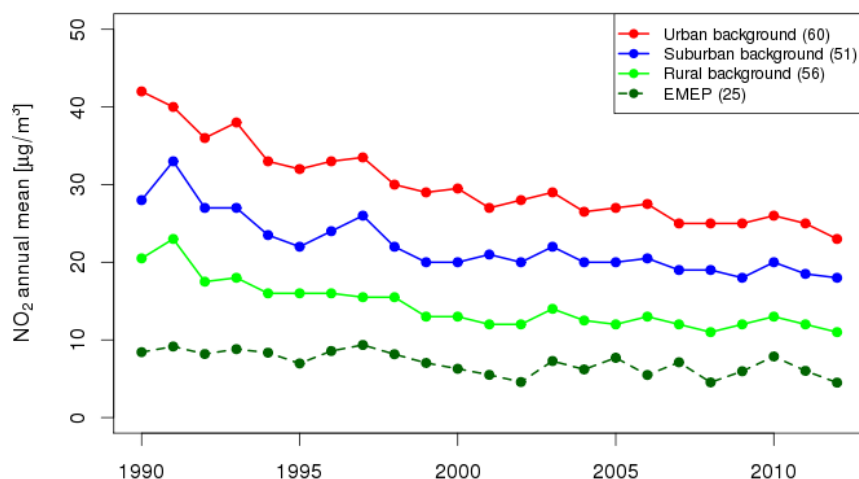
Figure 2.4: Median \text{NO}_2 time series ( \mu\text{g}/\text{m}^3 ) at EMEP and AIRBASE stations (for urban, suburban and rural background sites) passing the completeness criteria. For each type of site, the number of stations in the composite is given in the legend. Adapted from (Colette et al., 2015).
