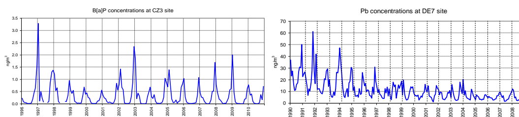
Figure B.1: Air concentrations of B[a]P and lead at EMEP sites CZ3 and DE7, 1990 – 2010, monthly means
