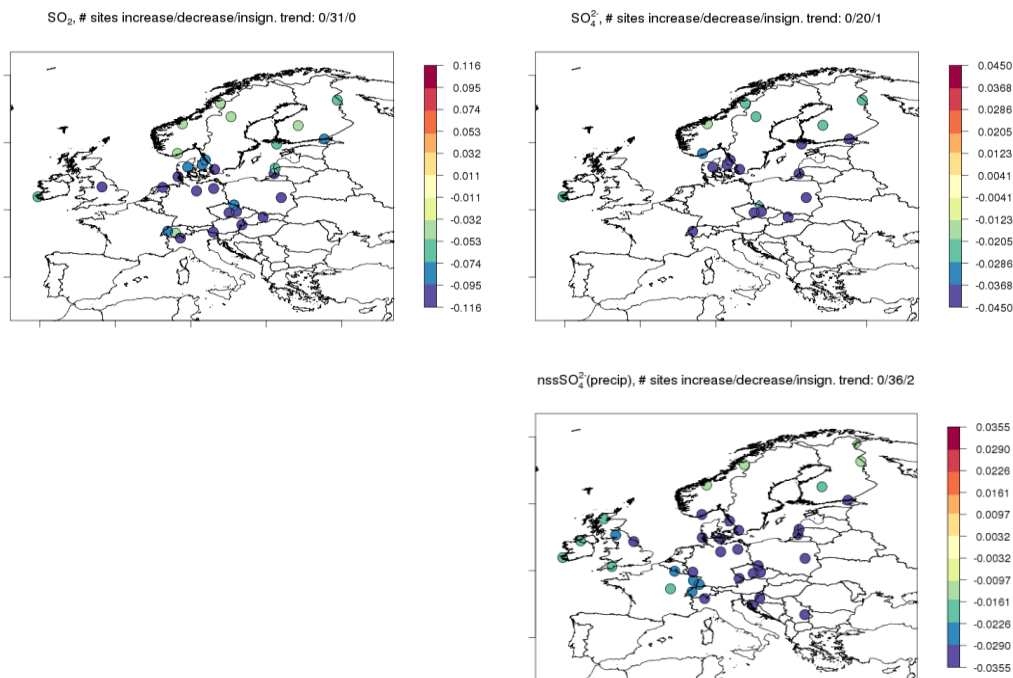
Figure 3.3: Maps of annual trends at EMEP sites over the 1990-2012 time period for gaseous sulfur dioxide (top left), particulate sulfate (top right) (in \mu\text{gS m}^{-3} \text{yr}^{-1} ) and sea-salt corrected sulfate concentration in precipitation (in \text{mgS L}^{-1} \text{yr}^{-1} ) (bottom right). Stations where the trend is significant at the 0.05 level are displayed with a circle, elsewhere a diamond is used.
