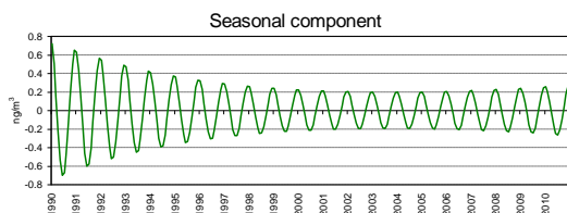
Figure B.4: Characterization of the seasonal component
