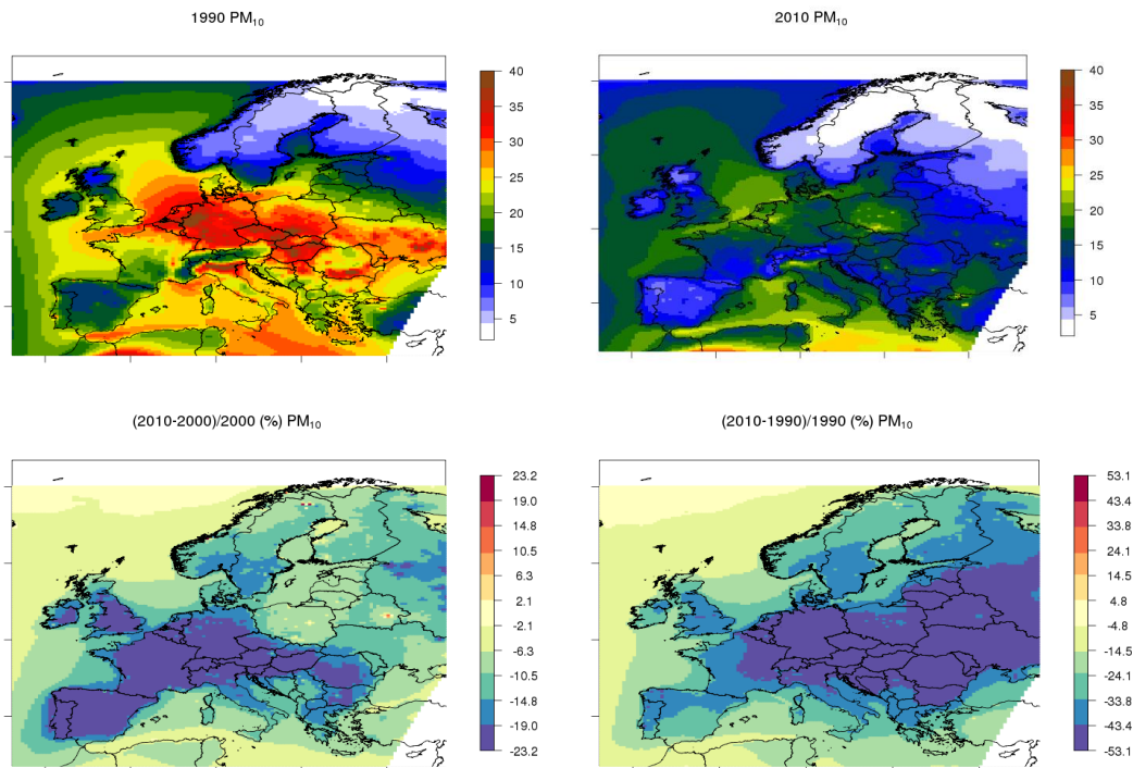
Figure 3.16: Modelled PM 10 ( \mu\text{g}/\text{m}^3 ) from the EURODELTA 6-model ensemble using 1990 (top left) or 2010 (top right) emissions and relative change (%) between 2000 and 2010 (bottom left) and 1990 and 2010 (bottom right).
