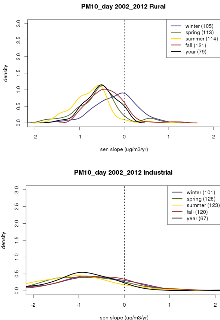
Figure 3.12: Distribution of PM_{10} trends over the 2002-2012 period for the four seasons and the annual trends in rural background stations (upper panel) and industrial sites (lower panel). The number in brackets shows the number of sites in the distributions.
