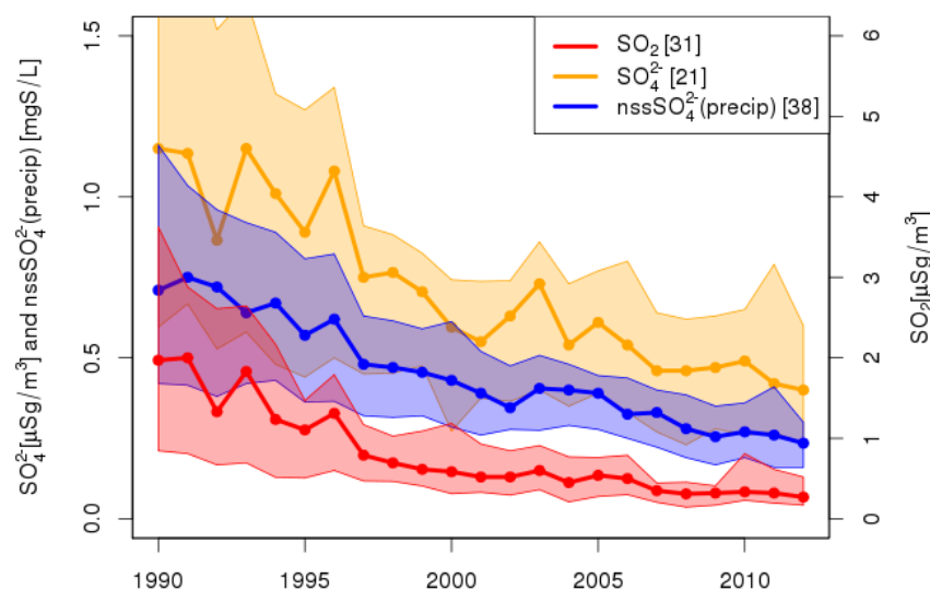
Figure 3.2: Median time series across the EMEP network and 25 th and 75 th quantiles over 1990-2012 for annual mean concentrations of gaseous sulfur dioxide (SO 2 ), particulate sulfate (SO 4 2- ), and sulfate concentration in precipitation excluding sea-salt (nssSO 4 2-(precip) ). The number of stations contributing to the median differ but, over time, a consistent set passing completion criteria is used for each compound.
