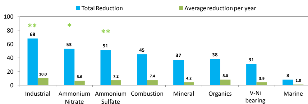
Figure 3.14: Total reduction and average reduction per year (in %) of PM mass from the 8 sources, detected from PMF analysis, explaining the gravimetric \text{PM}_{2.5} mass measured in the period 2002 – 2012 at Montseny station (Spain). Green symbols highlight the statistically significance of the trends following the Mann-Kendall test: *** ( p -value < 0.001), ** ( p -value < 0.01), * ( p -value < 0.05). No star means no statistically significant trend at p < 0.05 confidence level over the considered period.
