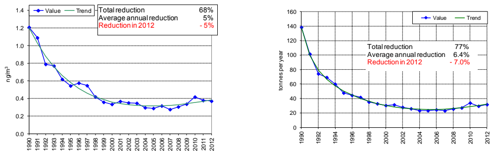
Figure 4.13: Trends of modelled annual mean air concentrations (a) and emissions (b) in Germany for the period from 1990 to 2012. Reduction rates refer to general trend. Negative reduction denotes increase of air concentrations.
