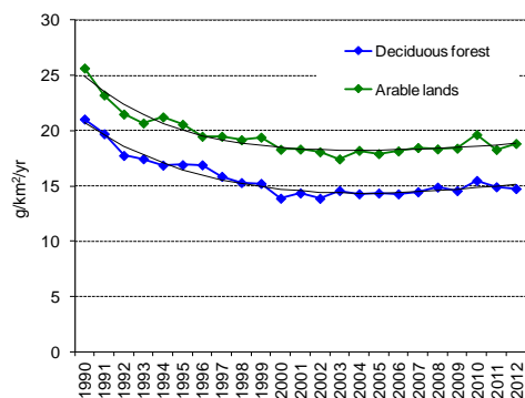
Figure 4.10: Trends of modelled B[a]P deposition to deciduous forest and arable lands within the EMEP region.
