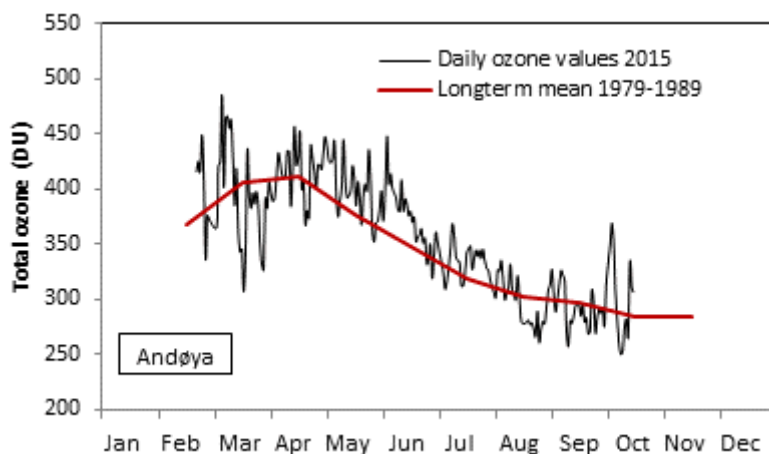
Figure 2a: Daily total ozone values measured at ALOMAR, Andøya, in 2015 by the Brewer and GUV instruments (black curve). The red line is the long-term monthly mean values from 1979-1989.
