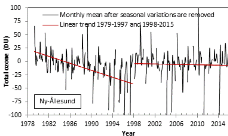
Figure 6b: Variations in total ozone at Ny-Ålesund for the period 1979-2015. Only data for the months March-September are included.
