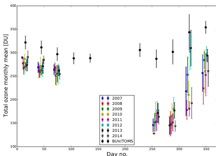
Figure 12: Monthly mean total ozone as measured with the Troll Station NILU-UV instrument, including the standard deviation of daily values considered (shown as error bars). BUV/TOMS monthly means: based on 1970 - 1981 satellite measurements
