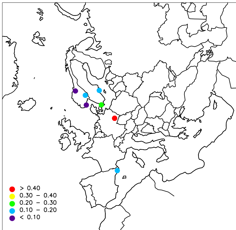
Figure 1.13: Geographical distribution of EC in PM 10 2014. Unit: \mu\text{g}/\text{m}^3 .
