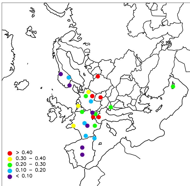
Figure 1.14: Geographical distribution of EC in PM 2.5 2014. Unit: \mu\text{g}/\text{m}^3 .
