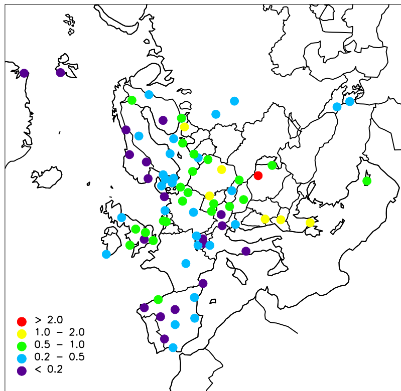
Figure 1.1: Geographical distribution of sulphur dioxide 2014. Unit: \mu\text{g S/m}^3 .
