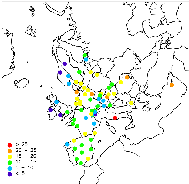
Figure 1.4: Geographical distribution of PM 10 2014. Unit: \mu\text{g}/\text{m}^3 .
