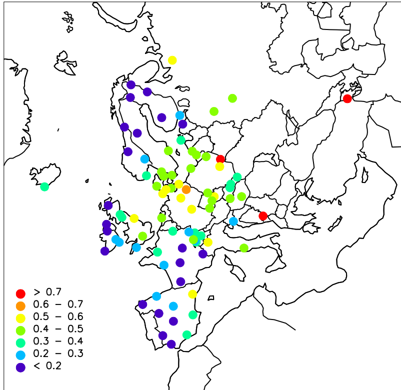
Figure 1.7: Geographical distribution of ammonium in precipitation 2014. Unit: mg N/l.
