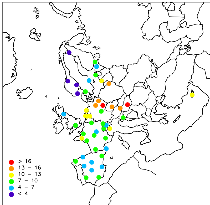
Figure 1.5: Geographical distribution of PM_{2.5} 2014. Unit: \mu g/m^3 .
