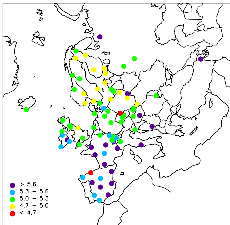
Figure 1.6: Geographical distribution of pH in precipitation 2014. Unit: pH units.
