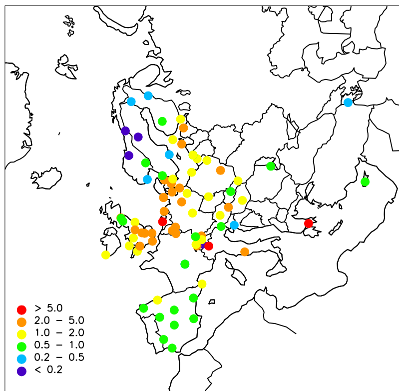
Figure 1.2: Geographical distribution of nitrogen dioxide 2014. Unit: \mu\text{g N/m}^3 .
