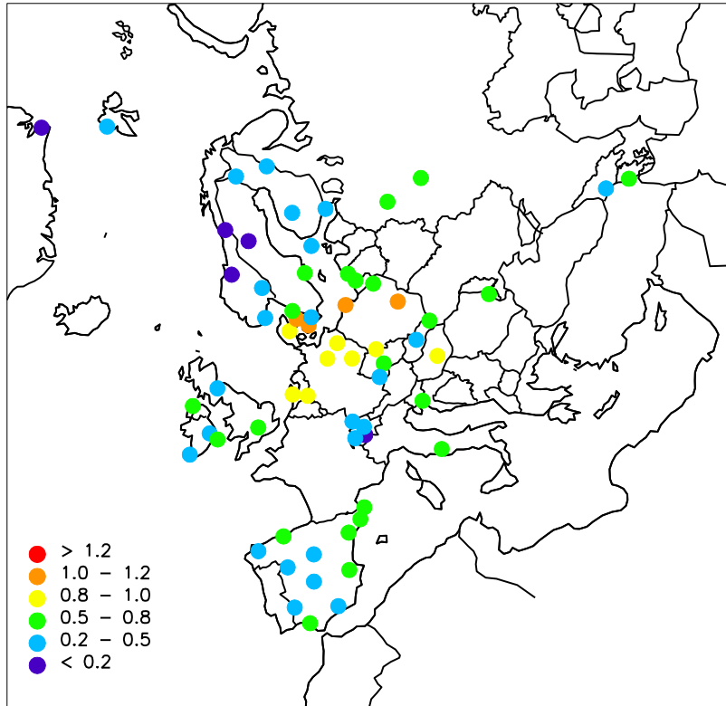
Figure 1.3: Geographical distribution of sulphate in aerosols 2014. Unit: \mu\text{g S}/\text{m}^3 .
