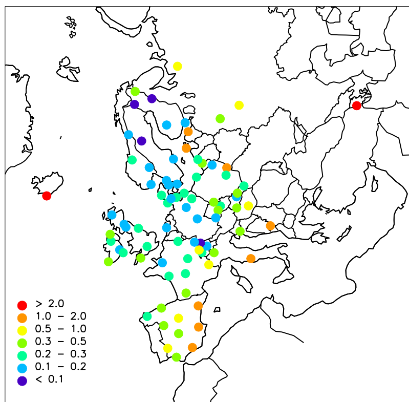
Figure 1.10: Geographical distribution of calcium in precipitation 2014. Unit: mg/l.
