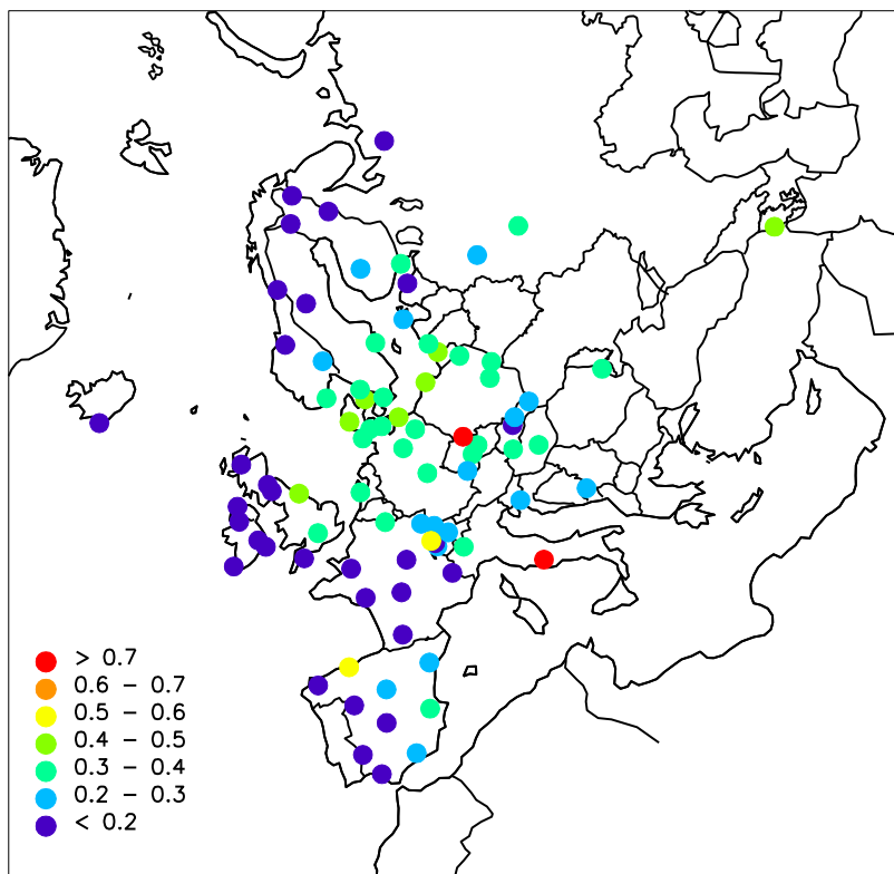
Figure 1.8: Geographical distribution of nitrate in precipitation 2014. Unit: mg N/l.
