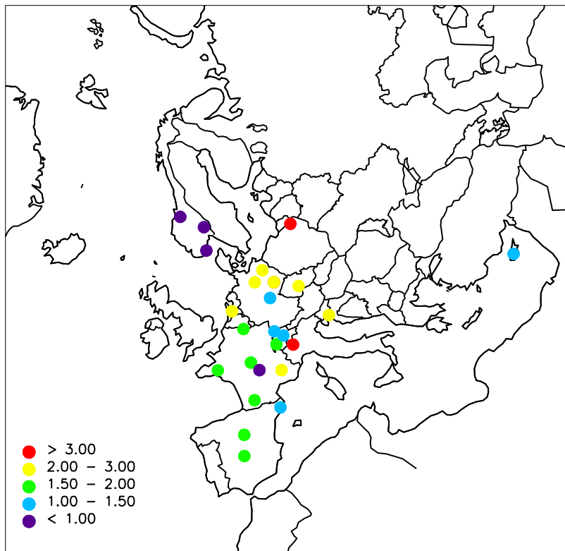
Figure 1.12: Geographical distribution of OC in PM 2.5 2014. Unit: \mu\text{g}/\text{m}^3 .
