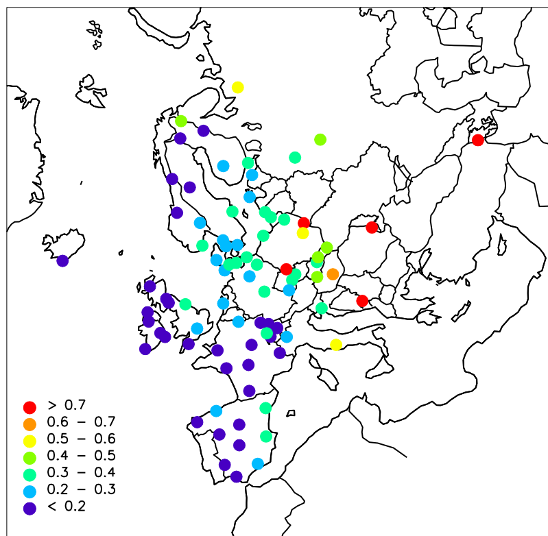
Figure 1.9: Geographical distribution of sulphate in precipitation 2014 (corrected for sea spray). Unit: mg S/l.
