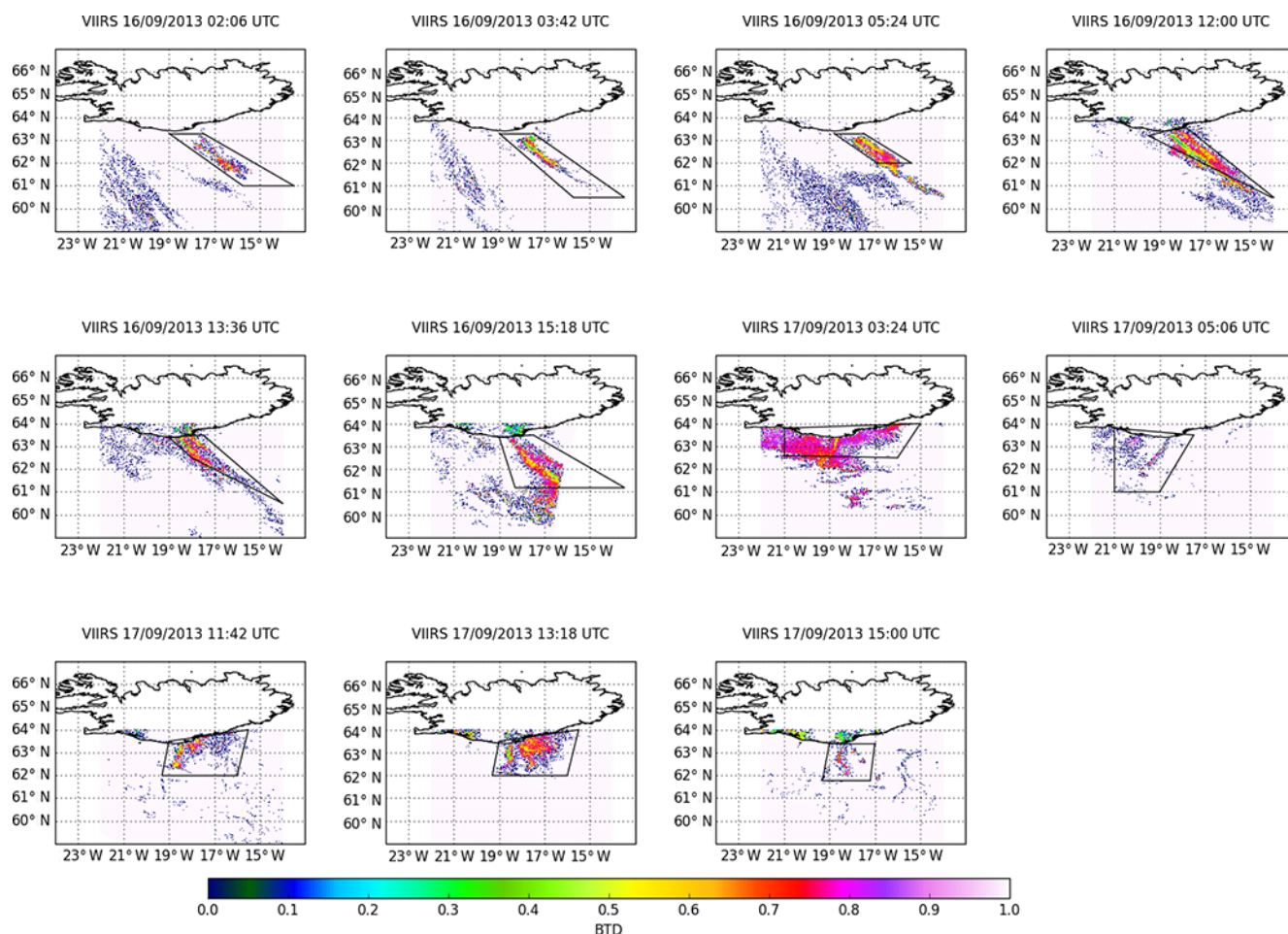
Figure 9. VIIRS BTs for pixels identified as resuspended ash, 16–17 September 2013.
