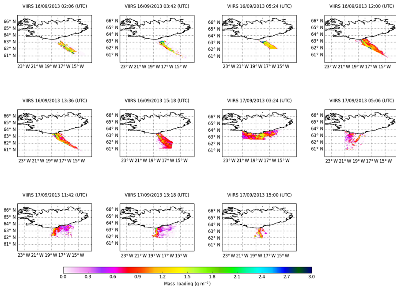
Figure 10. The resuspended ash mass loading retrieved from VIIRS infrared bands M15 and M16 for the areas identified as containing ash.
