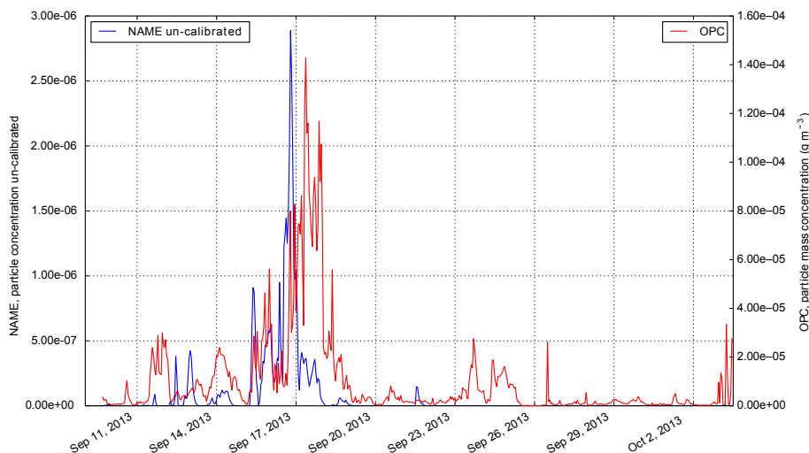
Figure 3. Time series of 1 h averaged concentrations of resuspended ash derived from OPC count data (red) compared to the un-calibrated modelled air concentrations (blue) at Marúbakki during September 2013.
