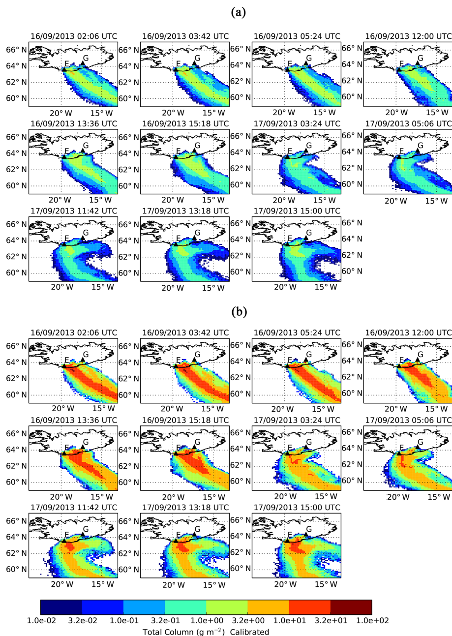
Figure 12. Modelled 1 h averaged total column mass loadings ( \text{g m}^{-2} ), where the source strength in NAME is calibrated using the scaling coefficient determined from the peak-to-peak scaling to the satellite-retrieved total column values (a) K = 1 \times 10^3 and (b) K = 1 \times 10^4 . The locations of the volcanoes Eyjafjallajökull and Grímsvötn are indicated on the map by the E and G symbols respectively.
