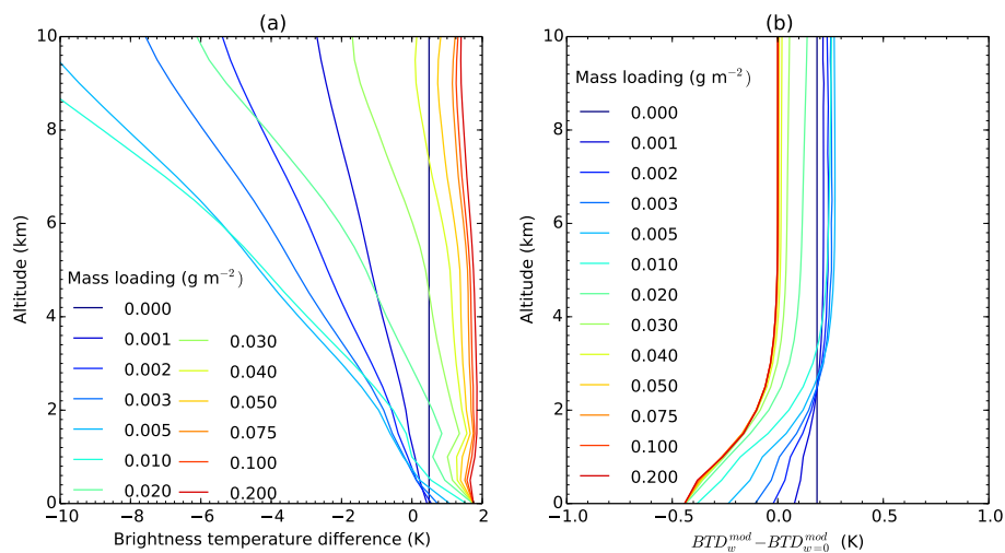
Figure 8. (a) The simulated brightness temperature difference between VIIRS bands M15 and M16, BTD_V , for a 1 km thick ash layer as a function of ash layer top altitude. (b) The difference BTD_W^{mod} - BTD_{W=0}^{mod} as a function of ash cloud top height. The curves represent varying ash mass loading ( \text{g m}^{-2} ) and are given in the legend.
