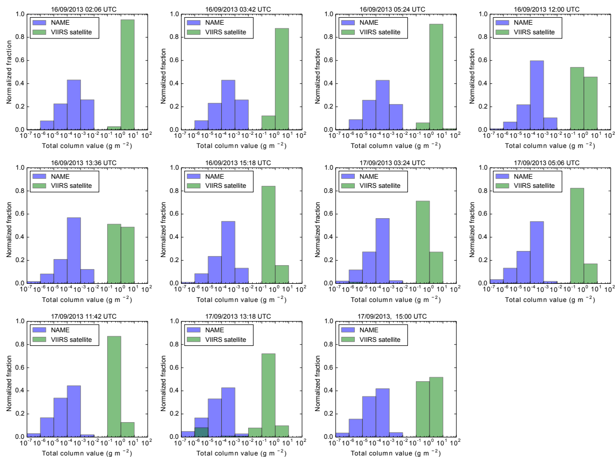
Figure 11. Comparing the frequency of binned total column mass loadings of the resuspended ash cloud modelled using NAME with an un-calibrated source strength to those retrieved from VIIRS during 16–17 September 2013.
