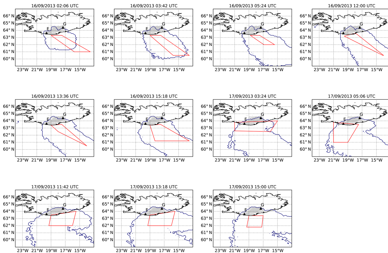
Figure 5. Comparison of the location of the modelled resuspended ash cloud, represented by the blue line, to the area identified from VIIRS retrieval data, represented by the red polygons; see Sect. 3.3 for the methodology used to define this area. The outline of the modelled plume is derived from un-calibrated 1 h averaged total column mass loadings; values > 10^{-7} \text{ g m}^{-2} are considered. The source areas are identified by the grey areas.
