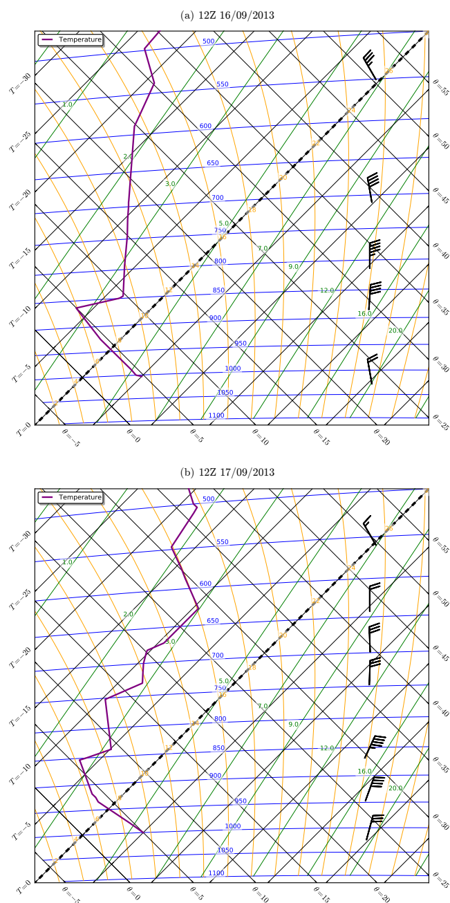
Figure 2. Radiosonde data retrieved from launches at Keflavík Airport at 12:00 UTC on (a) 16 and (b) 17 September 2013. North-westerly surface winds prevail on 16 September, and a temperature inversion is observed at 850 hPa, \sim 1500 \text{ m a.s.l.} (where pressure is indicated by the blue lines). On 17 September surface winds have veered north-easterly; the temperature inversion remains although it is now weaker. Radiosonde data were obtained from http://weather.uwyo.edu/upperair/sounding.html .
