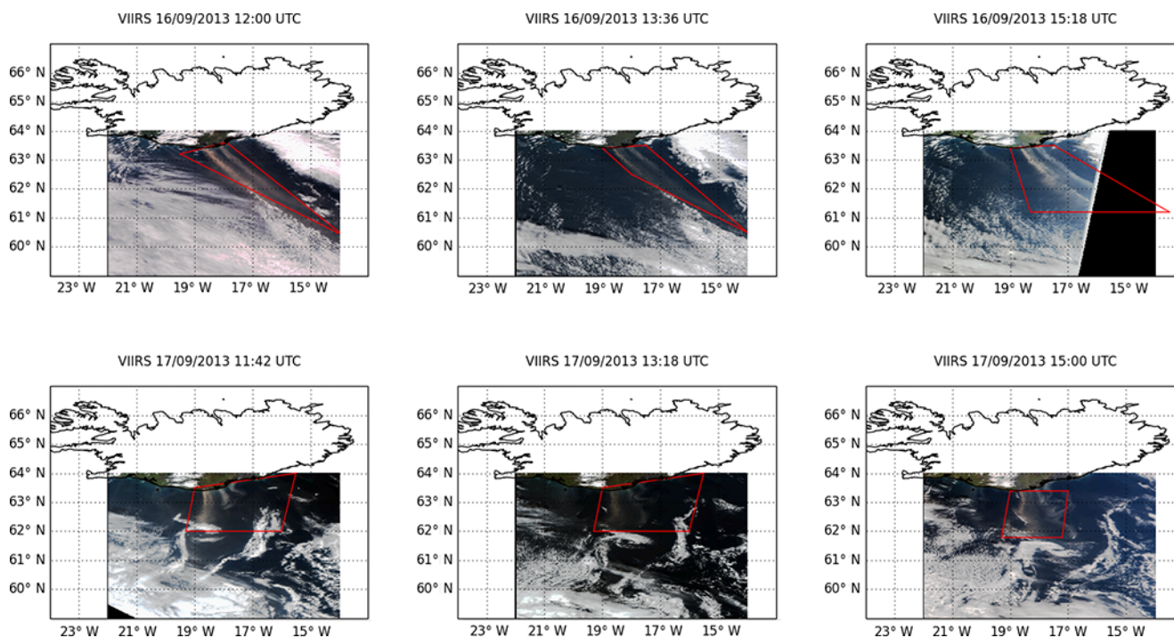
Figure 4. VIIRS daytime RGB composites using bands M3, M4, and M5 for 16–17 September 2013. Areas identified as containing resuspended ash (see Sect. 3.3) are enclosed within the red polygons.
