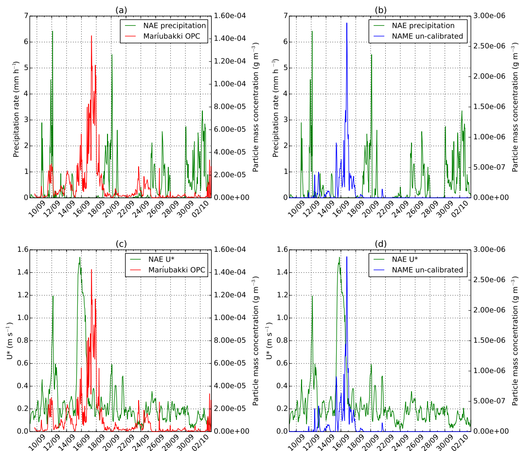
Figure 6. Time series of 1 h averaged air concentrations of resuspended ash derived from OPC count data and the un-calibrated model output, compared to the NAE precipitation rate and friction velocity ( U^* ) at Mariubakki.
