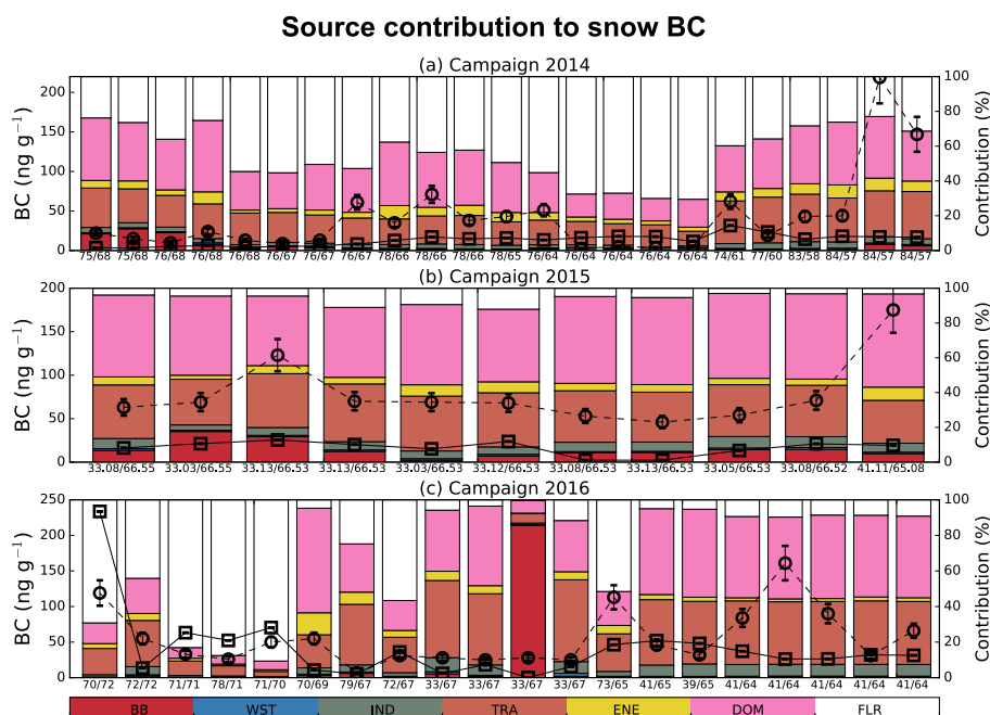
Figure 2. Contribution from the various emission categories considered in the ECLIPSE and GFED inventories to simulated BC concentrations in snow in (a) 2014, (b) 2015 and (c) 2016 in western Siberia and northwestern European Russia. BB stands for biomass burning, WST for waste burning, IND for industrial combustion and processing, TRA for surface transportation, ENE for emissions from energy conversion and extraction, DOM for residential and commercial combustion, and FLR for gas flaring. Bars show the relative source contribution (0–100 %, right axis) and are sorted, from left to right, from the northernmost to the southernmost measurement location (coordinates are reported on the bottom as longitude/latitude). Measured EC concentrations in snow are reported with open circles, whereas modelled BC is shown with open rectangles (left axis).
