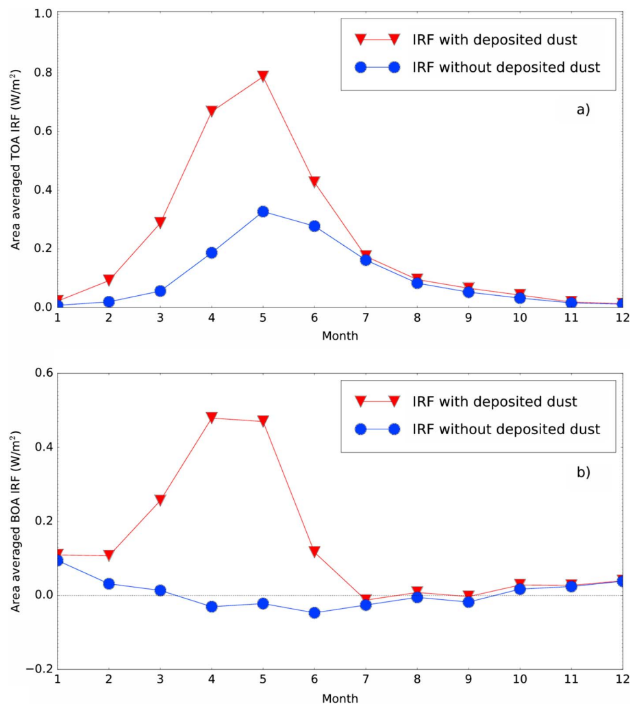
Figure 1. The area averaged (north of 60^\circ N ) dust (a) top of the atmosphere (TOA) and (b) bottom of the atmosphere (BOA) instantaneous radiative forcing (IRF) for 2012 conditions. The red (blue) curves show the IRF including (excluding) dust deposited on the surface. The black dotted line in panel (b) indicates the zero line.
