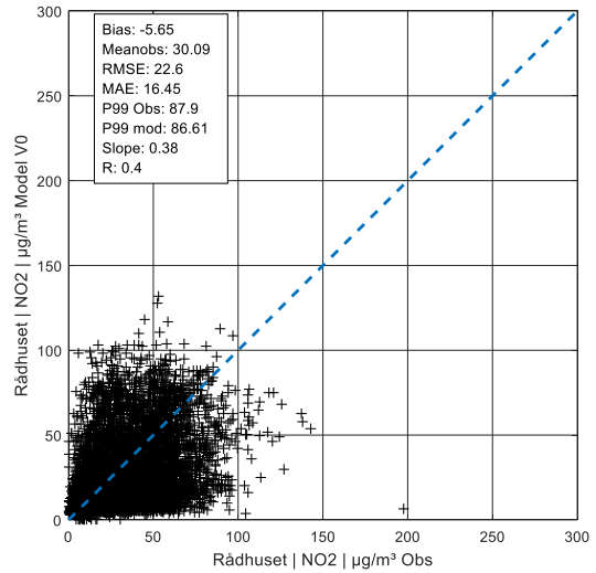
Figure A 6: Yearly value NO 2 in Rådhuset, V0
