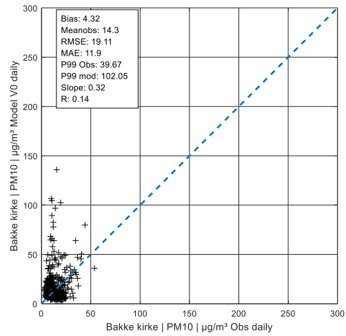
Figure A 200: Daily values PM 10 in Bakke kirke, V0
