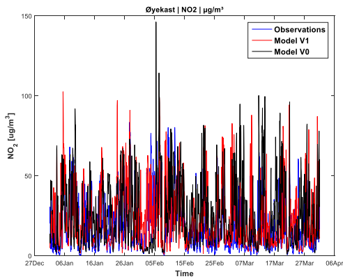
Figure A 44: Timesheet NO 2 in Øyekast
