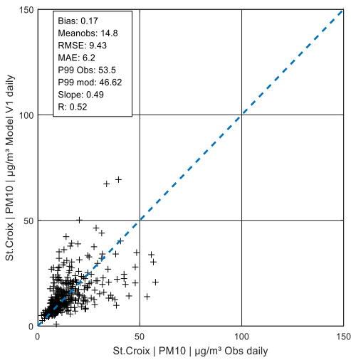
Figure A72: Daily value PM 10 in St. Croix, V1
