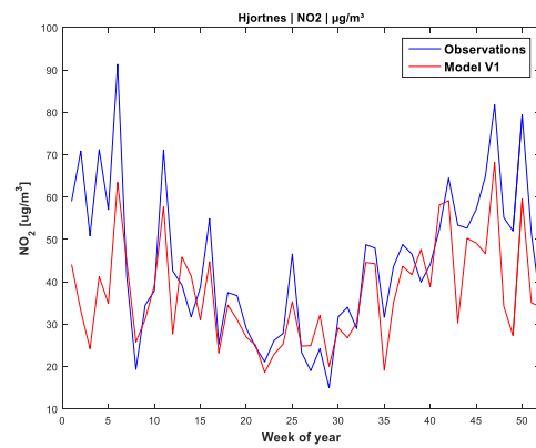
Figure A 94: Week of year NO 2 in Hjortnes, V1
