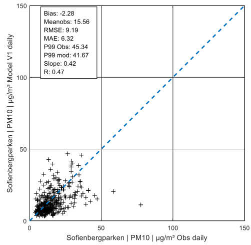
Figure A 132: Daily value PM 10 in Sofienbergparken, V1
