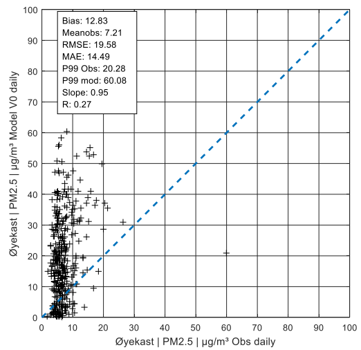
Figure A 64: Daily values PM 2.5 in Øyekast, V0
