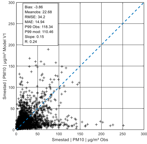
Figure A 128: Hourly values PM 10 in Smestad, V1 Figure A 129: Daily values PM 10 in Smestad, V1
