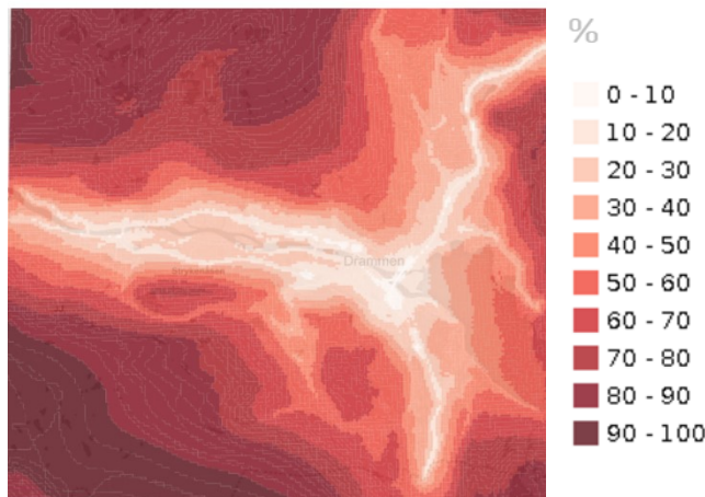
Figure 3.5.1: Percentage contribution from background air concentrations to the annual mean air pollution levels of \text{NO}_2 in Drammen in 2015. Units: Percentage [%]
