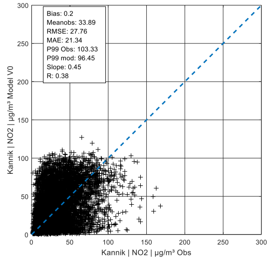
Figure A 162: Hourly values NO 2 in Kannik, V0
