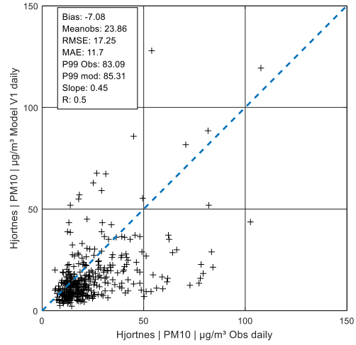
Figure A 116: Hourly values PM 10 in Hjørtnes,V1 Figure A 117: Daily values PM 10 in Hjørtnes,V1
