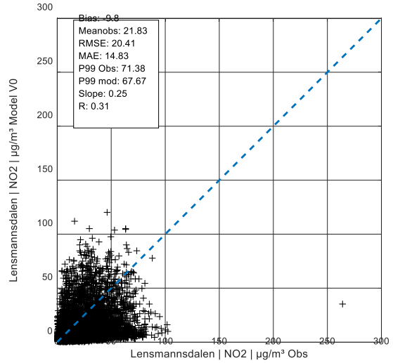
Figure A 39: Yearly value NO 2 in Lensmannsdalen, V0
