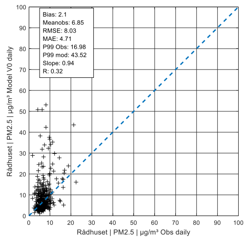
Figure A 27: Daily value PM 2.5 at Rådhuset, V0
