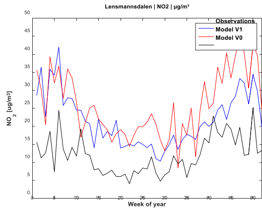
Figure A 41: Week of year NO 2 in Lensmannsdalen
