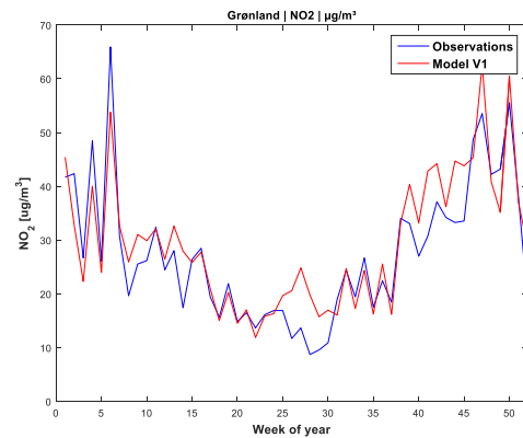
Figure A 91: Week of year NO 2 in Grønland, V1
