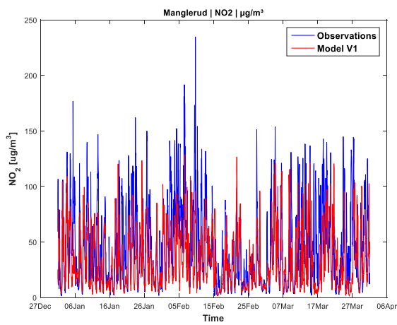
Figure A 99: Timeset NO 2 in Manglerud, V1
