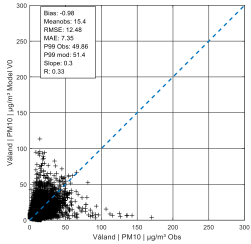
Figure A 175: Hourly values PM 10 in Våland, V0
