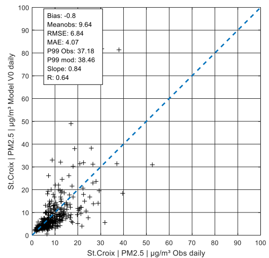
Figure A 78: Daily value PM 2.5 in St. Croix, V0
