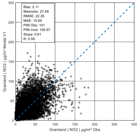
Figure A 89: Yearly value NO 2 in Grønland, V1
