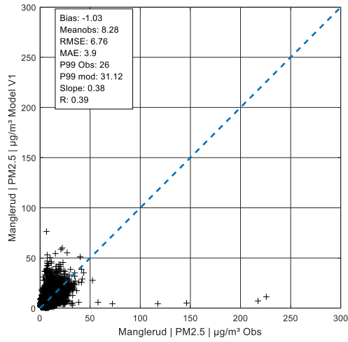
Figure A 149: Hourly values PM 2.5 in Manglerud, V1 Figure A 150: Daily values PM 2.5 in Manglerud, V1
