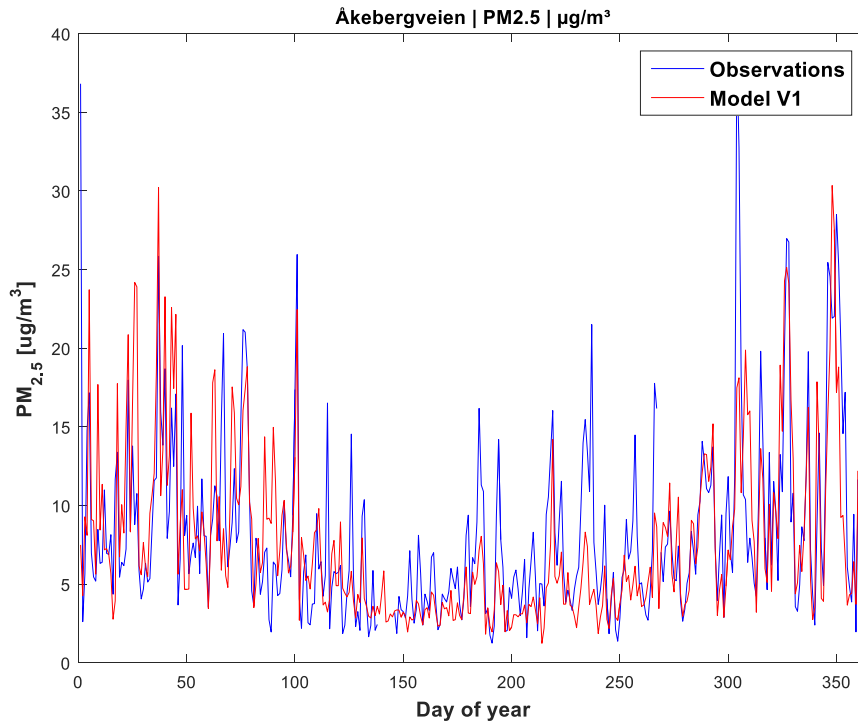
Figure A 136: Day of year PM 2.5 in Åkebergveien
