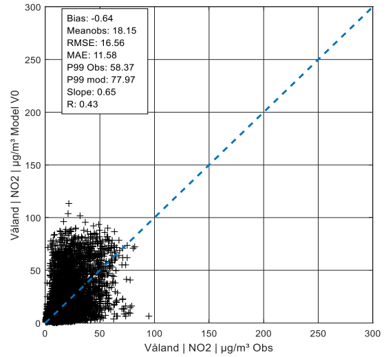
Figure A 166: Hourly values NO 2 in Våland, V0
