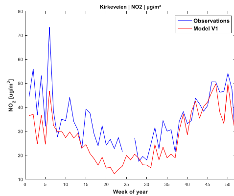
Figure A 97: Week of year NO 2 in Kirkeveien, V1
