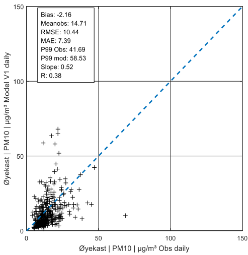
Figure A 53: Daily value PM 10 in Øyekast, V1
