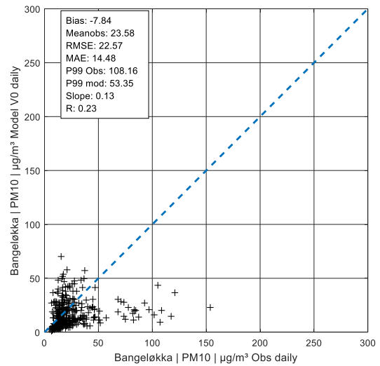
Figure A 36: Daily values PM 10 in Bangeløkka, V0
