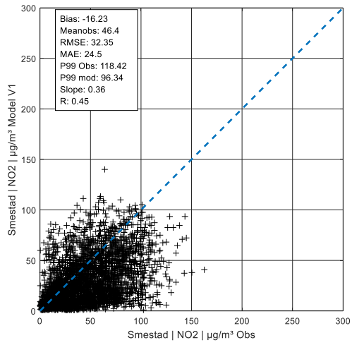
Figure A 104: Yearly value NO 2 in Smestad, V1
