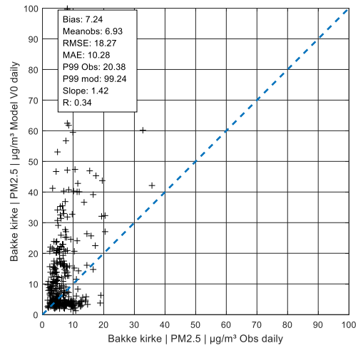
Figure A 210: Daily value PM 2.5 Bakke kirke, V0
