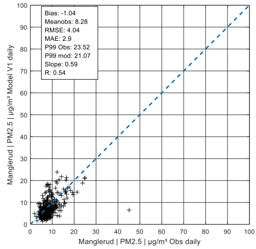
Figure A 149: Hourly values PM 2.5 in Manglerud, V1 Figure A 150: Daily values PM 2.5 in Manglerud, V1
