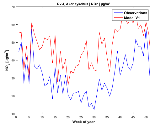
Figure A 103: Week of year NO 2 in Aker sykehus, V1
