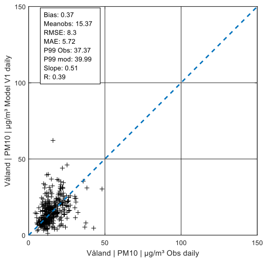
Figure A 176: Daily values PM 10 in Våland, V1
