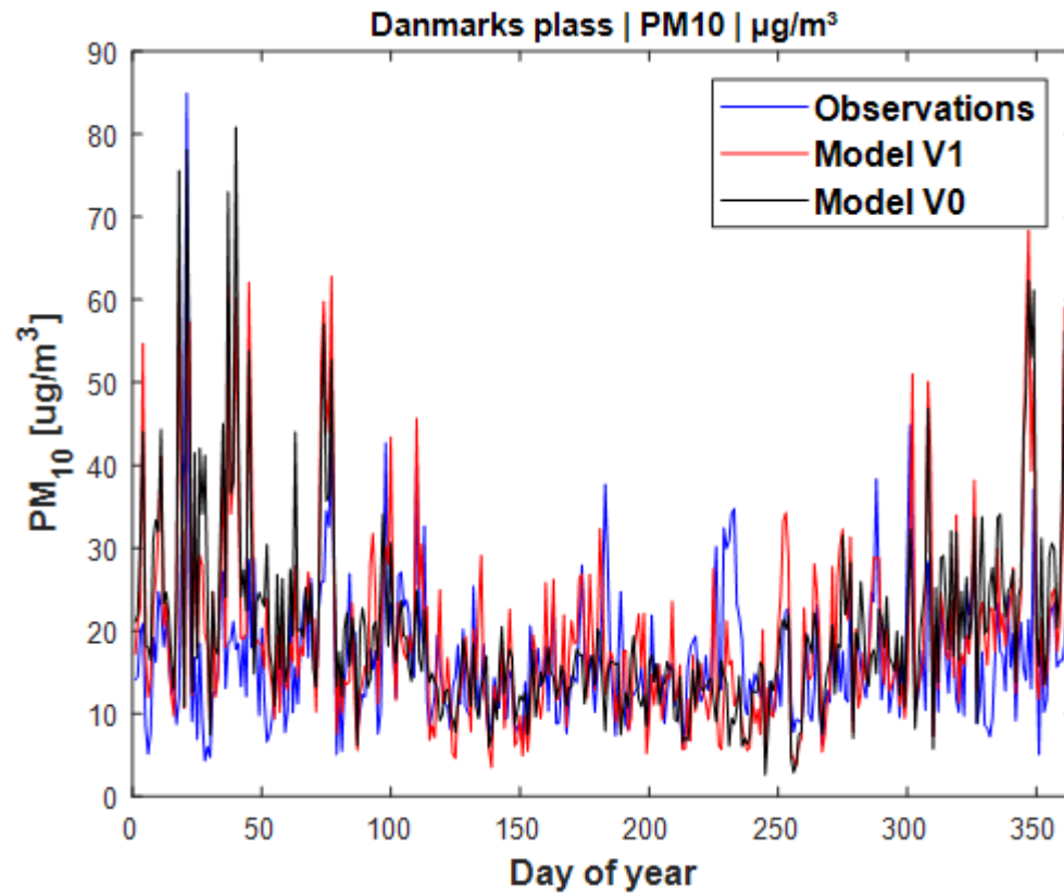
Figure A 13: Day of year PM 10 in Danmarks plass
