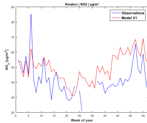
Figure A 85: Week of year NO 2 in Alnabru, V1
