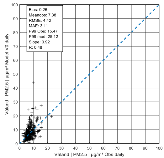
Figure A 187: Daily values PM 2.5 in Våland, V0
