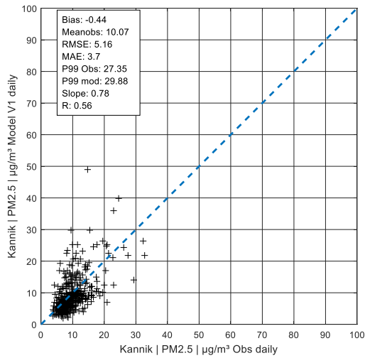
Figure A 181: Daily values PM 2.5 in Kannik, V1
