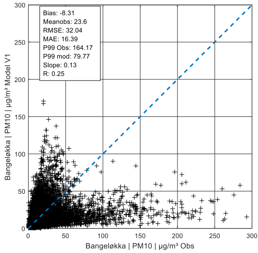
Figure A 33: Hourly values PM 10 in Bangeløkka, V1
