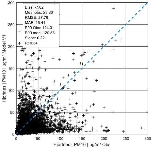
Figure A 116: Hourly values PM 10 in Hjørtnes,V1 Figure A 117: Daily values PM 10 in Hjørtnes,V1
