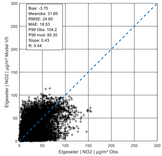
Figure A 194: Hourly values NO 2 in Elgeseter, V0
