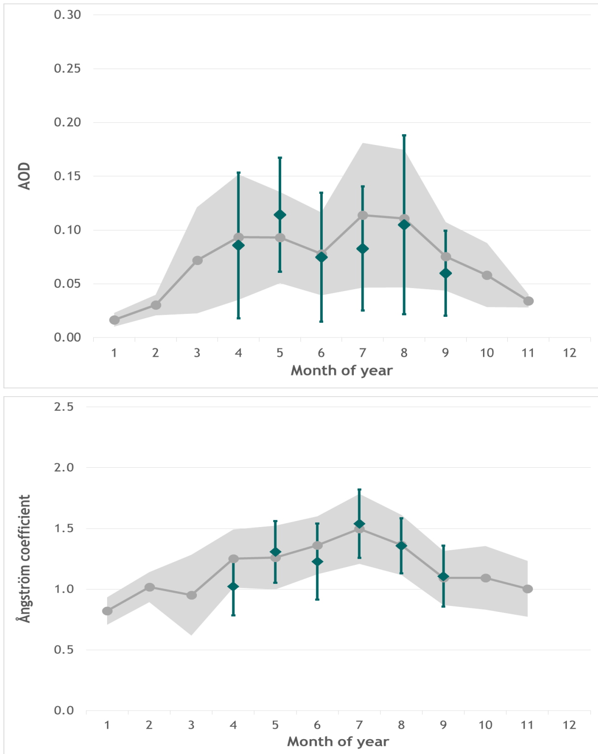
Figure 57: Monthly mean aerosol optical depth (AOD) at 500 nm wavelength in the atmospheric column above Birkenes (upper panel) and (470, 800 nm) Ångström coefficient describing the AOD wavelength dependence (lower panel). Mean values and standard deviations are given. Values marked in grey are the mean and standard deviations for the time period 2009-2018.
