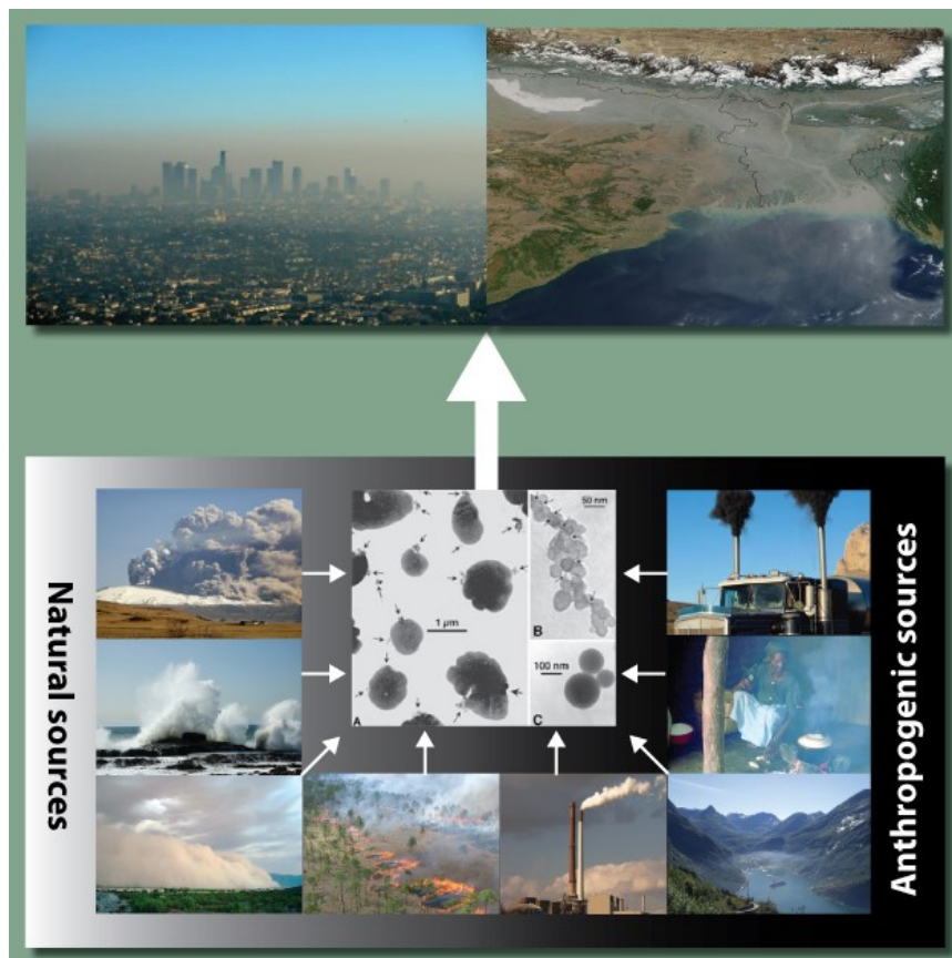
Figure 44: Illustration of the main natural and anthropogenic sources of atmospheric aerosols taken from Myhre et al (2013b). Top: local and large scale air pollution. Sources include (bottom, counter clockwise) volcanic eruptions (producing volcanic ash and sulphate), sea spray (sea salt and sulphate aerosols), desert storms (mineral dust), savannah biomass burning (BC and OC), coal power plants (fossil fuel BC and OC, sulphate, nitrate), ships (BC, OC, sulphates, nitrate), cooking* (domestic BC and OC), road transport (sulphate, BC, VOCs yielding OC). Additionally, Biogenic VOC to SOA and primary biological (e.g. pollen) from vegetation is crucial. Center: Electron microscope images of (A) sulphates, (B) soot, (C) fly ash, a product of coal combustion (Posfai et al., 1999).
