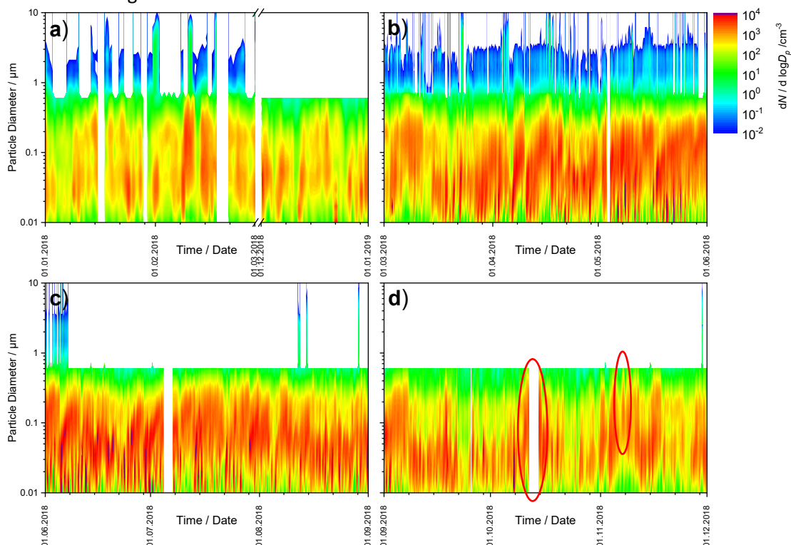
Figure 48: 2018 time series of particle number size distribution at Birkenes, panel a) winter, panel b) spring, panel c) summer, panel d) autumn. Episodes in autumn 2018 are marked by red oval shapes.
