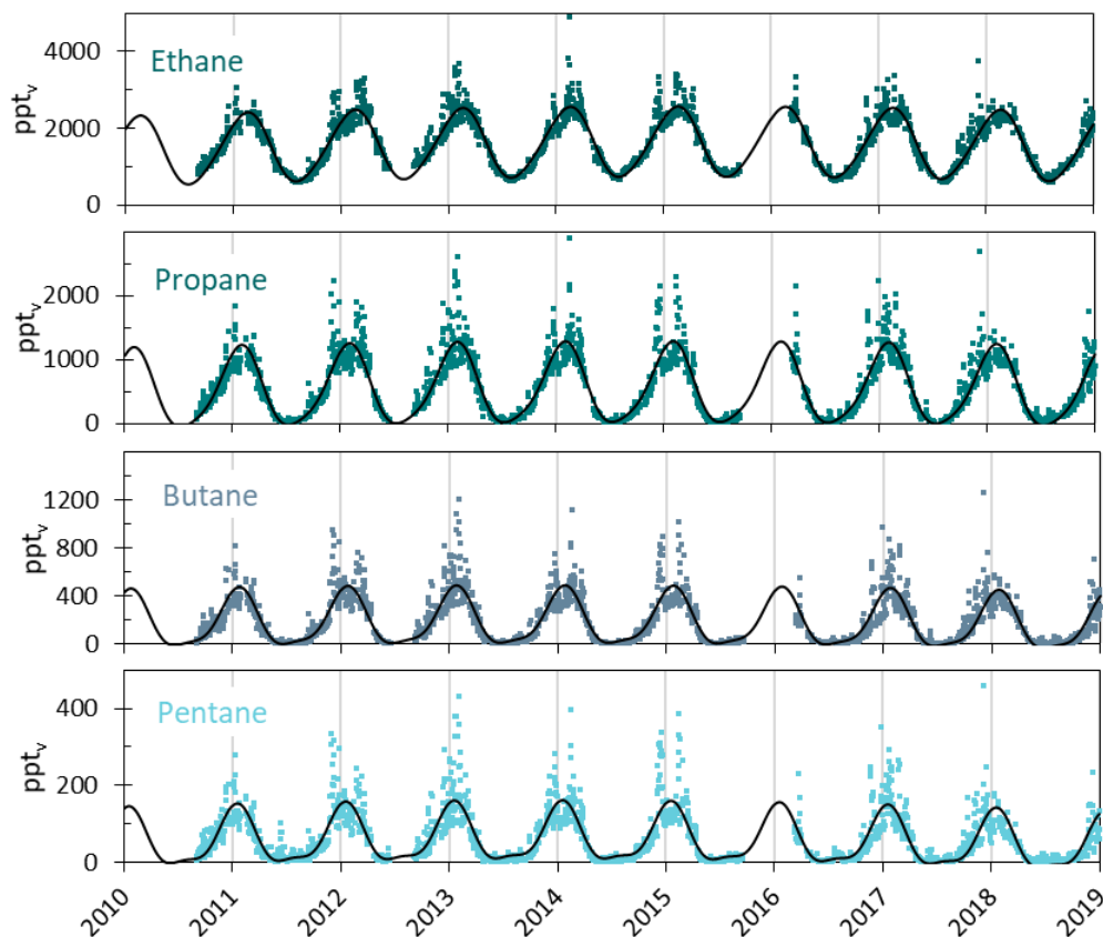
Figure 19: Observations of daily averaged mixing ratios of ethane, propane, butane, and pentane for the period September 2010 – 2018 at the Zeppelin Observatory.
