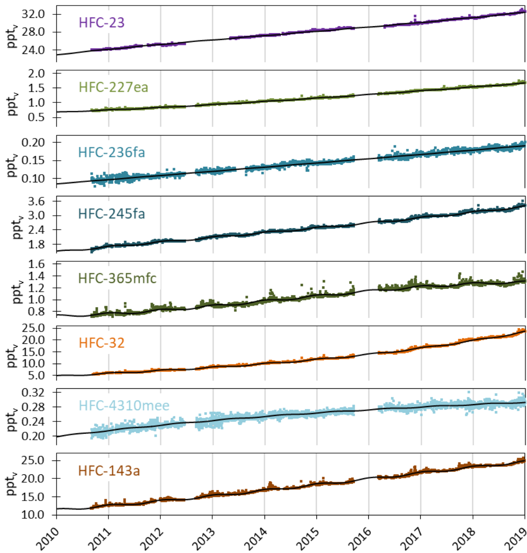
Figure 34: Daily averaged concentrations of monitored HFCs at the Zeppelin observatory for the period 2010-2018: HFC-23 (violet), HFC-227ea (light green), HFC-236fa (blue), HFC-245fa (dark blue), HFC-365mfc (dark green), HFC-32 (orange), HFC-4310mee (light blue), and HFC-143a (brown). The solid lines are empirical fitted mixing ratios.
