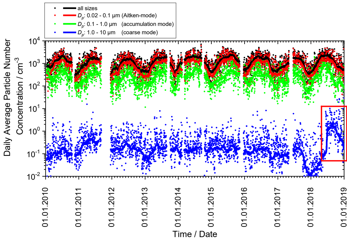
Figure 49: Birkenes 2010-2018 time series of particle number concentration integrated over selected size ranges representing the different physical processes governing the atmospheric aerosol. The dotted graphs represent daily averages of the respective size range, the lines the 8-week running median. The period where the OPSS, measuring the concentration of coarse size range particles, experienced calibration issues, is marked by a red box.
