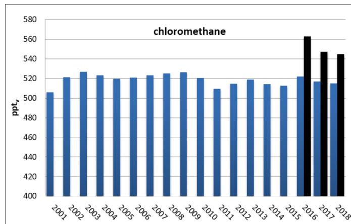
Figure 26: Development of Chloromethane annual means measured at the Zeppelin Observatory for the period 2001-2018. Global annual means for 2016-2018 are included as a black bars. All units are in pptv.
