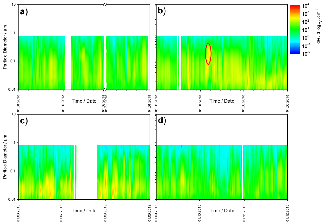
Figure 52: 2018 time series of particle number size distribution of the non-volatile particle fraction at Zeppelin, panel a) winter, panel b) spring, panel c) summer, panel d) autumn. An episode occurring around 6-7 April 2018 is marked with a red oval.
