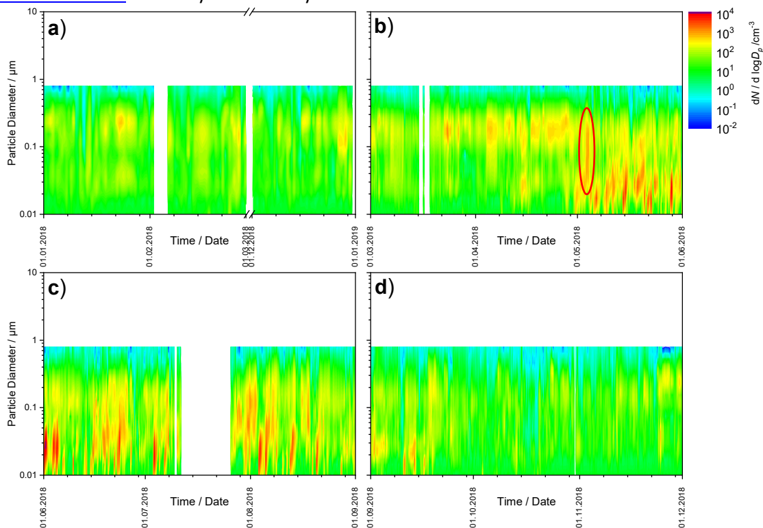
Figure 50: 2018 time series of particle number size distribution at Zeppelin, panel a) winter, panel b) spring, panel c) summer, panel d) autumn. An episode occurring around 3 May 2018 is marked with a red oval.
