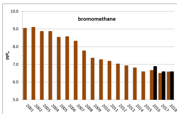
Figure 28: Development of the annual means of bromomethane measured at the Zeppelin Observatory for the period 2001-2018. The global annual mean for 2016-2018 are included as black bars.
