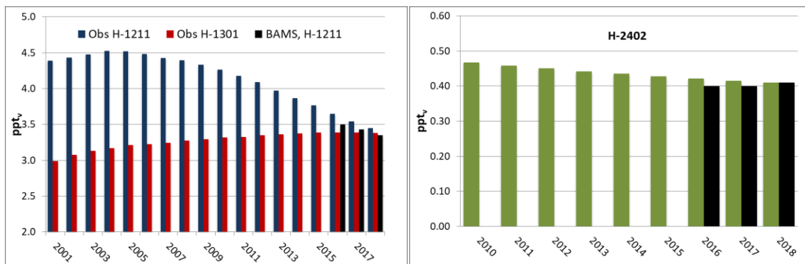
Figure 37: Development of the annual means of the observed halons at the Zeppelin Observatory. Red: H-1301, blue: H-1211, and green: H-2402. The global annual means in 2016, 2017 and 2018 are included as black bars. All units are in ppt.
