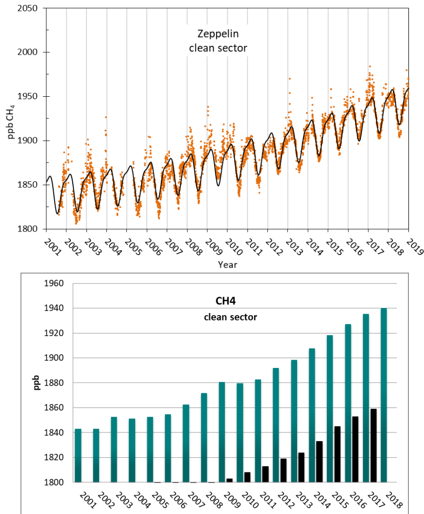
Figure 13: Upper panel: Daily mean CH 4 at Zeppelin for the days when the air comes from a clean sector (Arctic or north Atlantic). Lower panel; The annual mean, only taking days with clean air into account.
