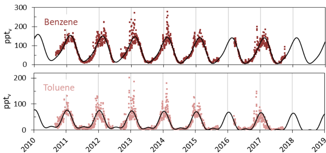
Figure 21: Observations of daily averaged mixing ratio of benzene (upper panel) and toluene (lower panel) for the period September 2010 – 2018 at the Zeppelin Observatory.
