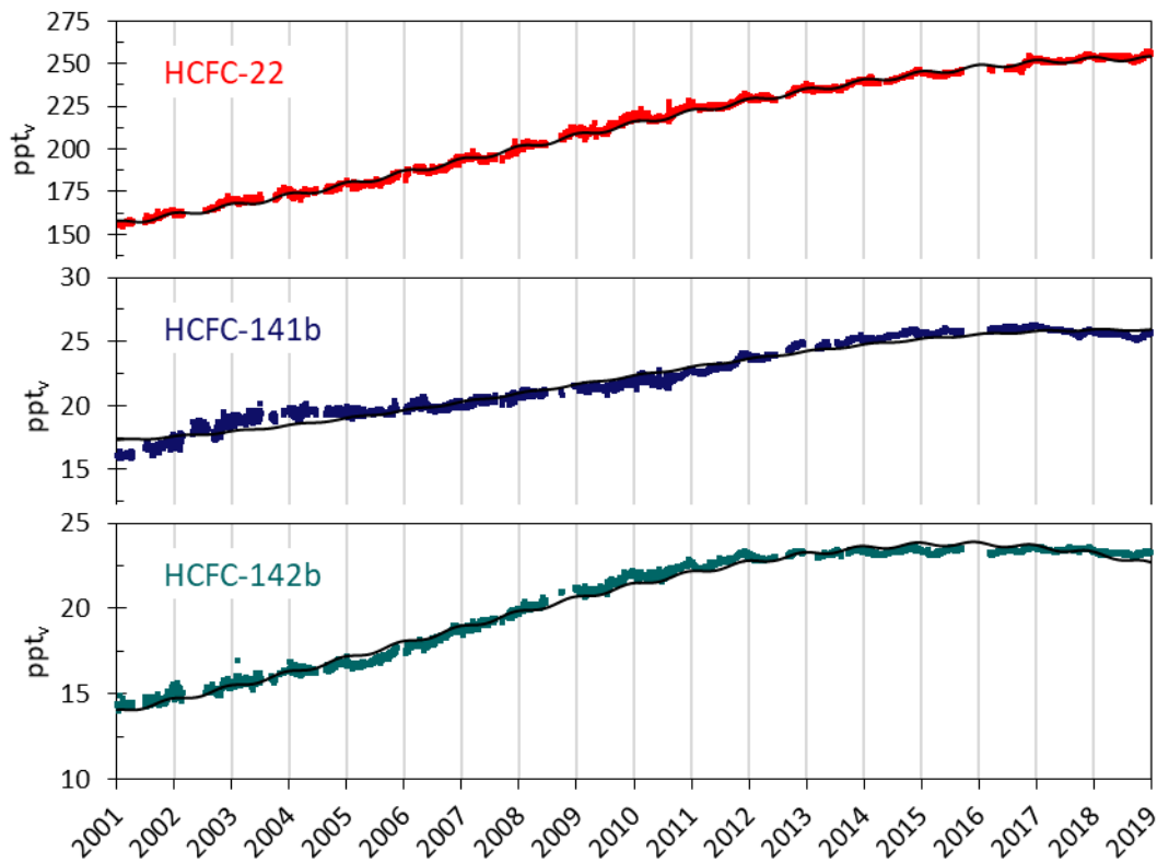
Figure 31: Daily averaged mixing ratios of the monitored HCFCs for the period 2001-2018 at the Zeppelin observatory: HCFC-22 (red), HCFC-141b (dark blue), and HCFC-142b (green). The solid lines are empirical fitted mixing ratios. All units are in ppt.
