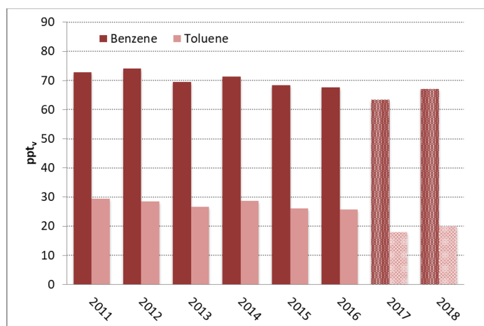
Figure 22: Development of the annual means of benzene (brown) and toluene (light red) for the period 2011 – 2018 at the Zeppelin Observatory. All concentrations are in ppt. Note that benzene and toluene in 2018 and second half of 2017 are based on model data only.
