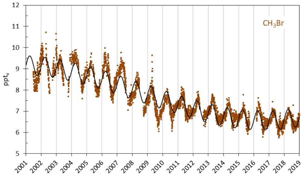
Figure 27: Observations of Bromomethane, \text{CH}_3\text{Br} , for the period 2001-2018 at the Zeppelin Observatory. Brown dots: daily averages mixing ratios from the observations, solid line empirical fitted mixing ratios.
