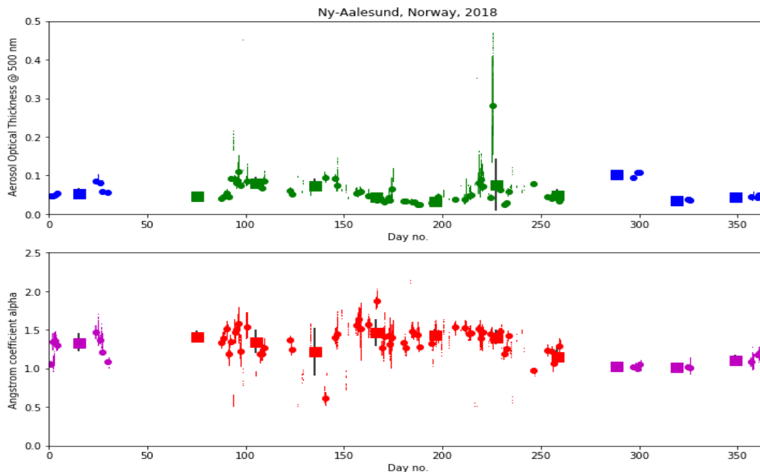
Figure 60: AOD and AE data, combining solar (green, red) and lunar (blue, magenta) observations. Single measurements are marked by dots, daily averages by filled circles and monthly means by filled squares. Standard deviations of single measurements used for means calculations are marked by error bars.
