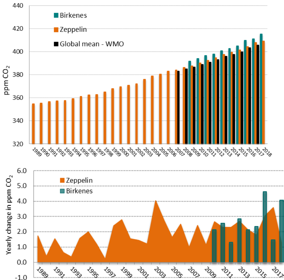
Figure 8: Upper panel: the annual mean concentrations of CO 2 measured at Zeppelin Observatory for the period 1989-2018 shown in orange. Prior to 2012, ITM University of Stockholm provides all data. The annual mean values from Birkenes are shown as green bars. The global mean values as given by WMO (2018) are included in black. The yearly annual changes are shown in the lower panel, orange for Zeppelin, green for Birkenes.
