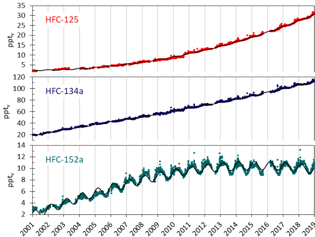
Figure 33: Daily averaged concentrations of the monitored HFCs for the period 2001-2018 at the Zeppelin observatory: HFC-125 (red), HFC-134a (dark blue), and HFC-152a (green). The solid lines are empirical fitted mixing ratios.
