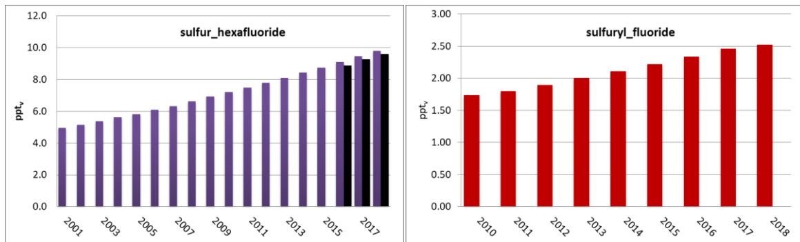
Figure 41: Annual means of SF 6 for the period 2001-2018 (left) and SO 2 F 2 for the period 2010-2018 (right) at the Zeppelin observatory. The global annual means for SF 6 in 2016 to 2018 are included as a black bars.
