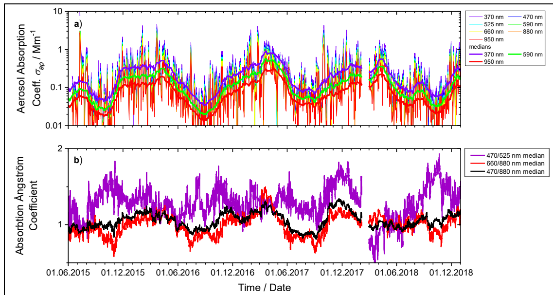
Figure 46: 2015 – 2018 time series graphs of data collected by the filter absorption photometer at Zeppelin Observatory since deployment in June 2015. Top: daily means of absorption coefficient at all 7 measured wavelengths (thin lines), and 8-week running medians for top, middle and bottom of observed spectral range (heavy lines). Bottom: 8-month running medians of absorption Ångström coefficient, top, bottom, and whole observed spectral range.
