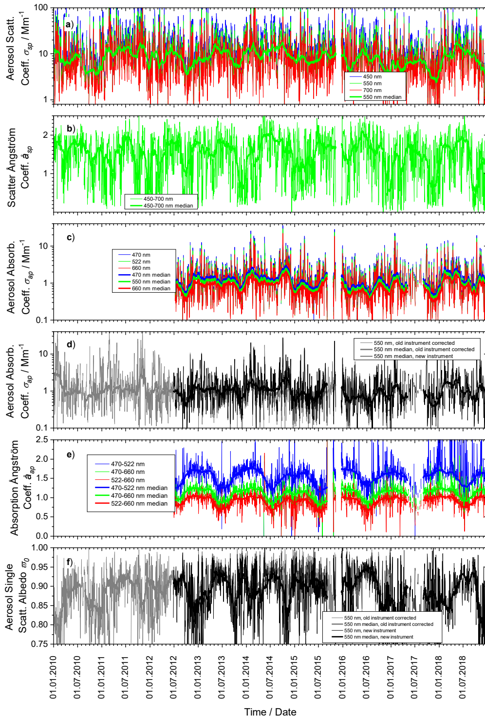
Figure 45: Time series of aerosol particle optical property daily means measured for 2010 - 2018 at Birkenes. Panel a) shows the aerosol scattering coefficient \sigma_{sp} at 450, 550, and 700 nm wavelength measured by integrating nephelometer. Panel c) the aerosol absorption coefficient \sigma_{ap} at 470, 522, and 660 nm wavelength measured by the newer filter absorption photometer, Panel d) the aerosol absorption coefficient \sigma_{ap} at 550 nm of the older filter absorption photometer, shifted from the instrument wavelength at 525 nm for consistent comparison assuming an absorption Ångström coefficient of -1. Panels b) and e) show the derived properties scattering and absorption Ångström coefficient \hat{a}_{sp} and \hat{a}_{ap} , respectively, while Panel f) depicts the single scattering albedo \omega_0 . All plots also depict the running 8-week medians of the respective properties as heavy lines to visualize seasonal
