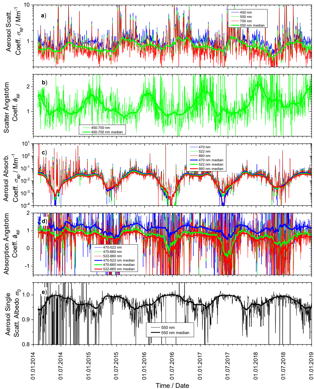
Figure 47: Time series of aerosol particle optical property daily means measured for 2014 - 2018 at Trollhaugen station. Panel a) shows the aerosol scattering coefficient \sigma_{sp} at 450, 550, and 700 nm wavelength measured by integrating nephelometer. Panel c) the aerosol absorption coefficient \sigma_{ap} at 470, 522, and 660 nm wavelength measured by filter absorption photometer. Panels b) and d) show the derived properties scattering and absorption Ångström coefficient \hat{a}_{sp} and \hat{a}_{ap} , respectively, while Panel e) depicts the single scattering albedo \omega_0 . All plots also depict the running 8-week medians of the respective properties as heavy lines to visualize seasonal variations.
