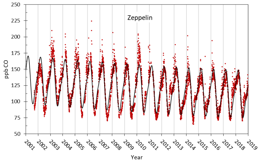
Figure 23: Observations of carbon monoxide (CO) from September 2001 to 2018 at the Zeppelin observatory. Red dots: daily averaged observed mixing ratios. The solid line is the empirical fitted mixing ratio.
