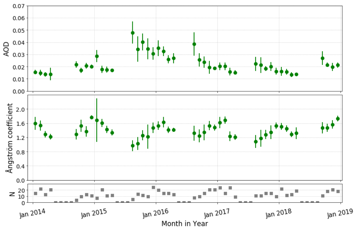
Figure 61: 2014 - 2018 time series of aerosol optical depth (AOD) at 500.5 nm wavelength in the atmospheric column above Trollhaugen Observatory, Antarctica (upper panel), Ångström coefficient (centre panel), and number of days per month with measurements. Monthly mean values and standard deviations are given
