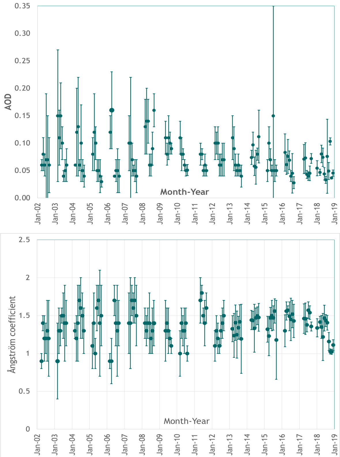
Figure 58: 2002 - 2018 time series of aerosol optical depth (AOD) at 500.5 nm wavelength in the atmospheric column above Ny-Ålesund (upper panel) and Ångström coefficient (lower panel). Monthly mean values and standard deviations are given.
