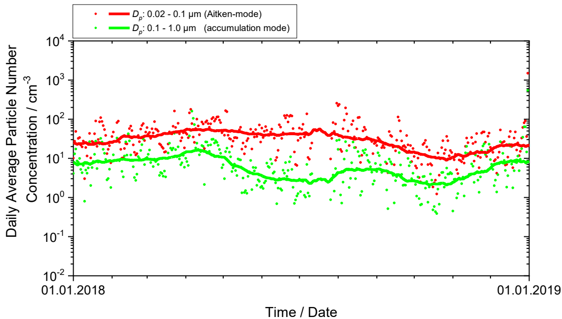
Figure 53: Zeppelin 2018 time series of number concentration in the refractory particle fraction integrated over selected size ranges representing the different physical processes governing the atmospheric aerosol. The dotted graphs represent daily averages of the respective size range, the lines the 8-week running median.
