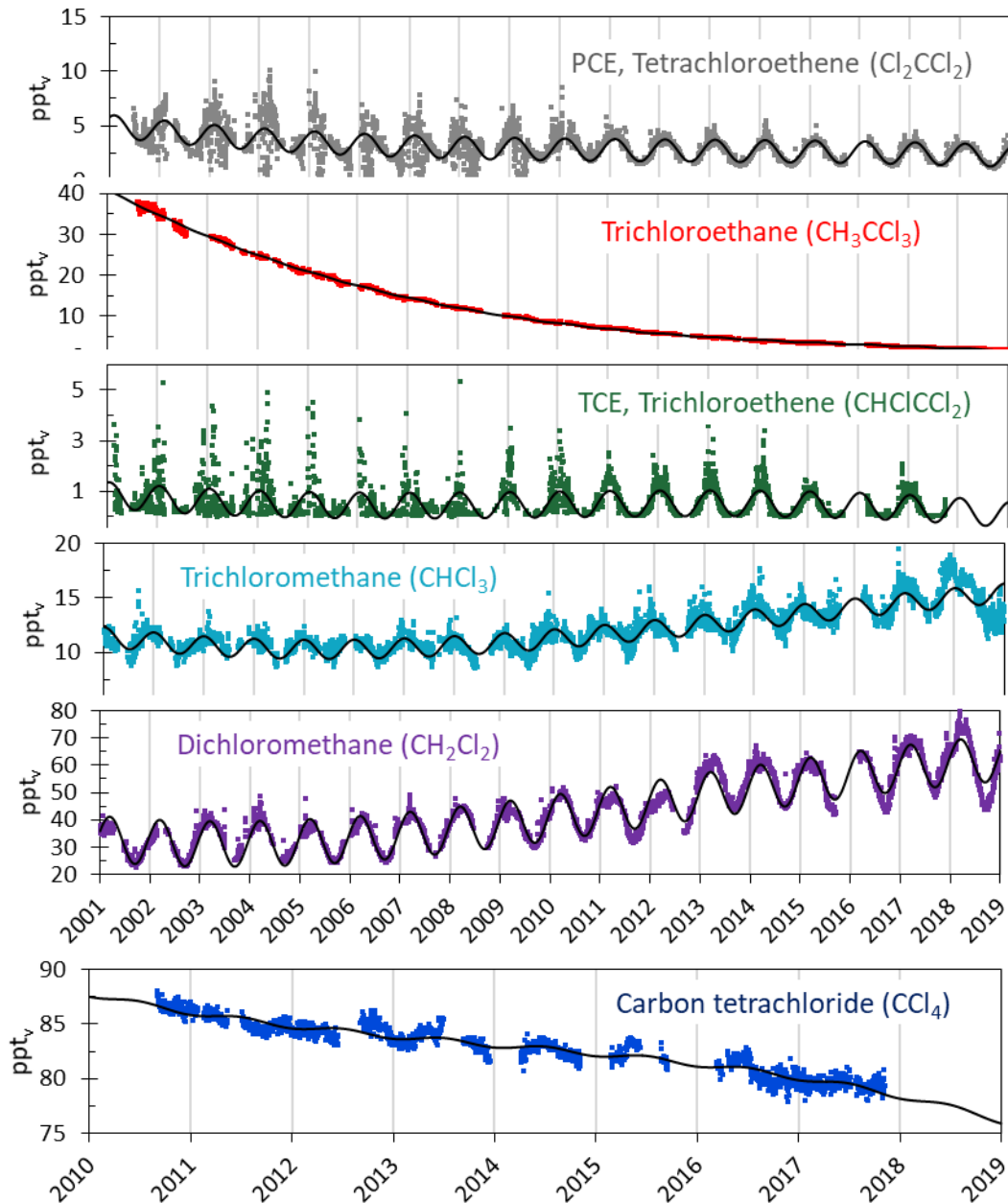
Figure 38: Daily averaged concentrations of chlorinated hydrocarbons at the Zeppelin observatory: For the period 2001-2018: Tetrachloroethene (grey), trichloroethane (red), trichloroethene (green), trichloromethane (light blue), and dichloromethane (violet). For the period 2010-2018: carbon tetrachloride (dark blue). Solid lines are empirical fitted mixing ratios.
