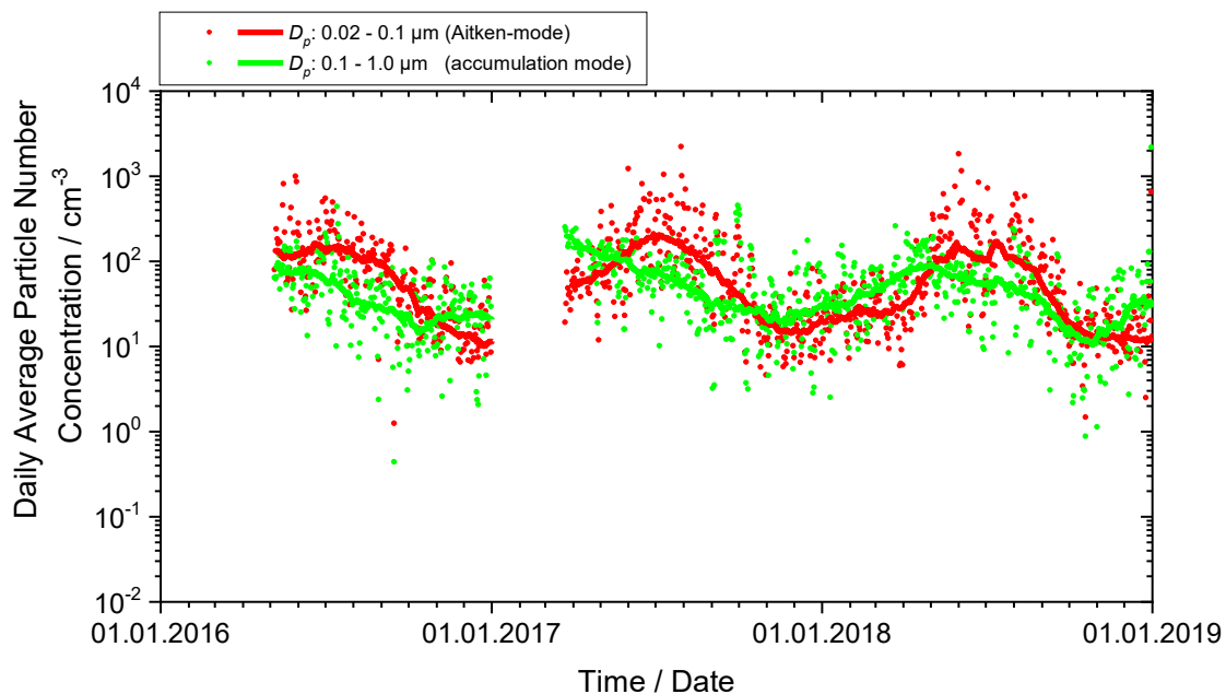
Figure 51: Zeppelin 2016-2018 time series of particle number concentration integrated over selected size ranges representing the different physical processes governing the atmospheric aerosol. The dotted graphs represent daily averages of the respective size range, the lines the 8-week running median.
