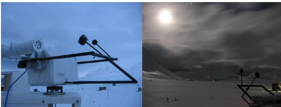
Figure 64: Moon PFR on the Kipp & Zonen tracker during the day (left, parking position) and during night-time measurements (right).
