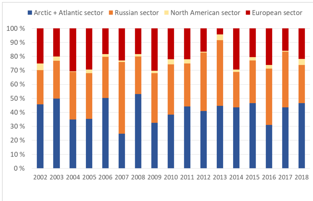
Figure 12: The percentage of polluted and clean air arriving at Zeppelin in the period 2002-2018 from the various sectors.
