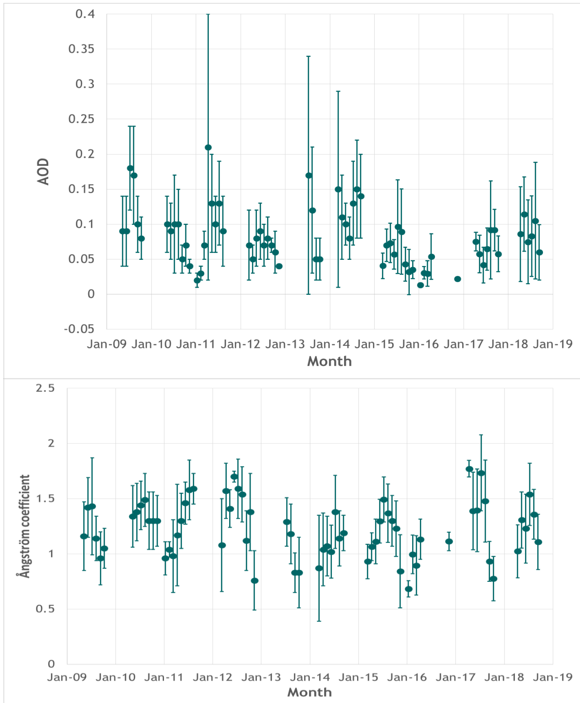
Figure 56: 2009 - 2018 time series of aerosol optical depth (AOD) at 500 nm wavelength in the atmospheric column above Birkenes (upper panel) and (470 nm, 800 nm) Ångström coefficient describing the AOD wavelength dependence (lower panel). Mean values and standard deviations are given
