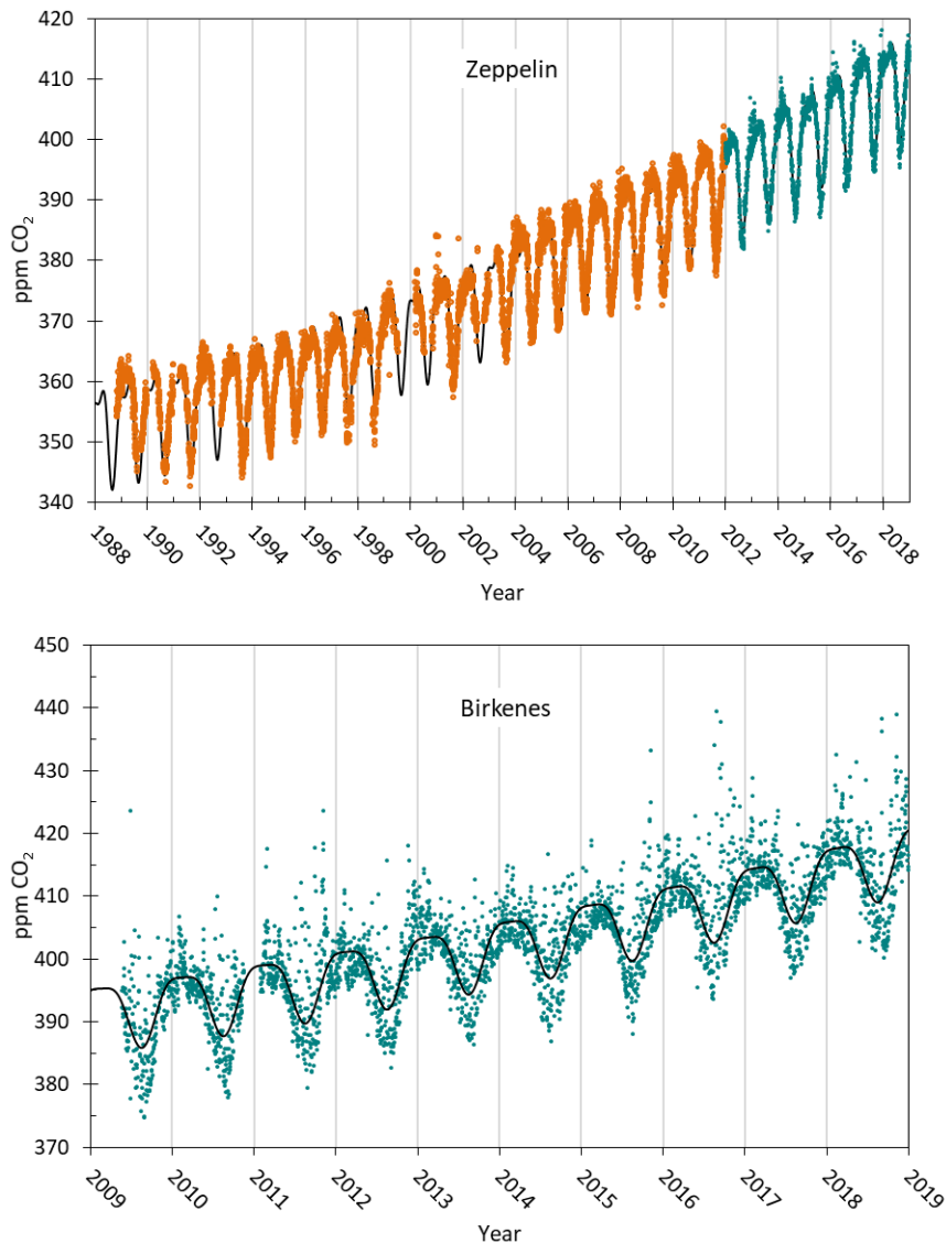
Figure 7: The atmospheric daily mean CO 2 concentrations measured at the Zeppelin Observatory for the period mid 1988-2018 are presented in the upper panel. Prior to 2012, ITM University of Stockholm provided all data, shown in orange. The green dots represent measurements from the Picarro instrument installed by NILU in 2012. CO 2 measurements at Birkenes are shown in the lower panel, the green dots are daily mean concentrations.
