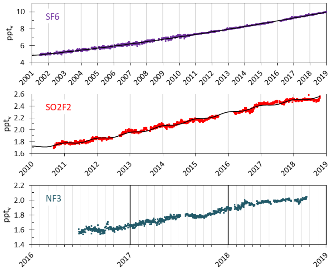
Figure 40: Daily averaged concentrations at the Zeppelin Observatory. Upper panel: \text{SF}_6 for the period 2001-2018. Middle panel: \text{SO}_2\text{F}_2 for the period 2010-2018. Lower panel: \text{NF}_3 from mid 2016 to 2018. Solid lines are statistical fitted mixing ratios.
