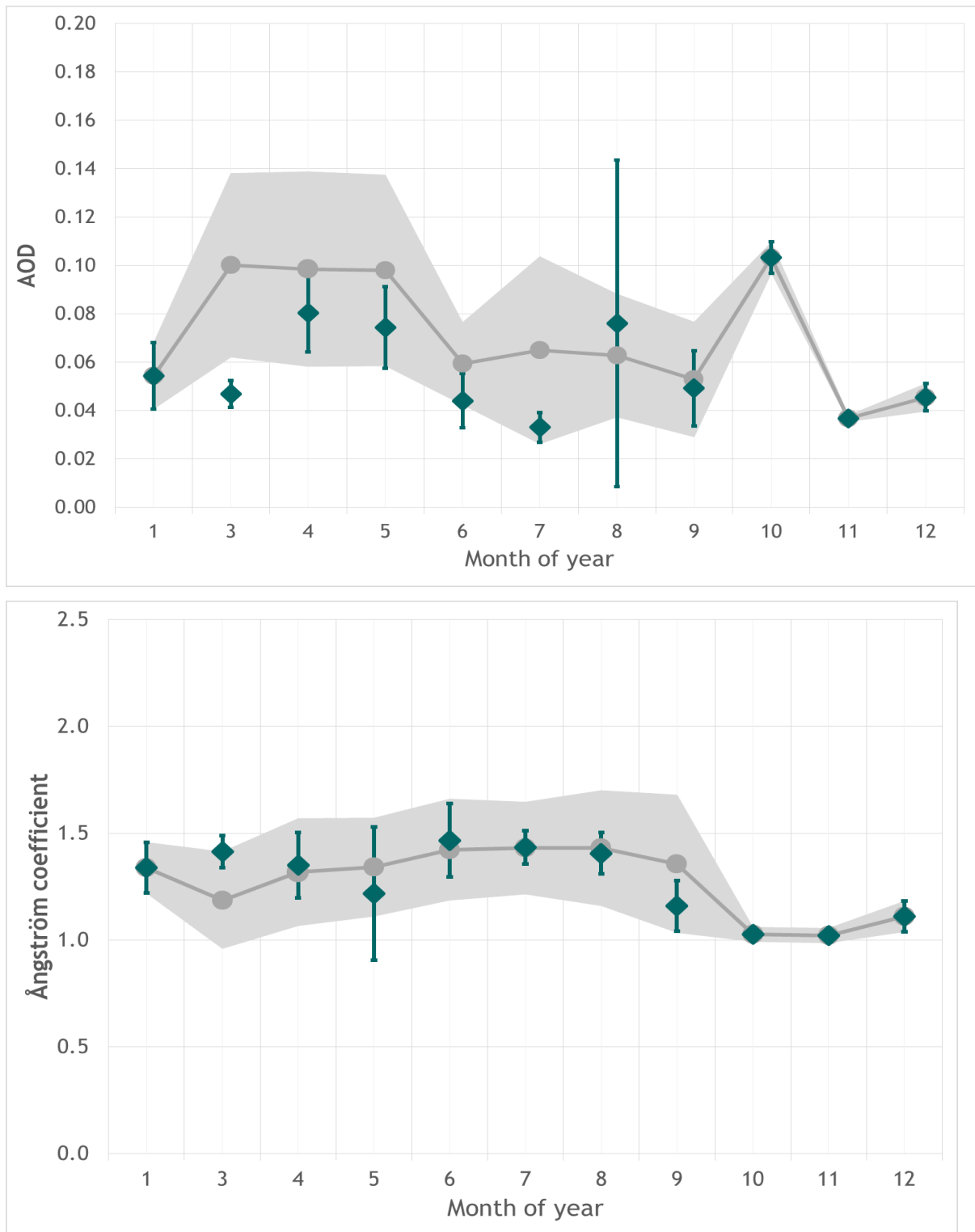
Figure 59: Seasonal variation of the aerosol optical depth (AOD) (upper panel) and Ångström coefficient (lower panel) observed in Ny-Ålesund. Values marked in grey are the mean and standard deviations for the time period 2009-2018; the 2018 monthly mean and standard deviations are shown in green.
