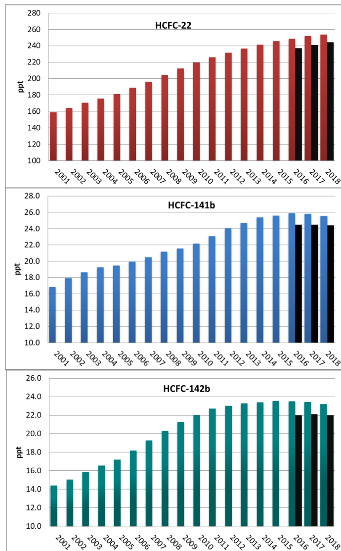
Figure 32: Development of the annual means of observed HCFCs at the Zeppelin Observatory for the period 2001-2018. HCFC-22 (red), HCFC-141b (blue), and HCFC-142b (green). The global annual means in 2016, 2017 and 2018 are included as black bars. All units are in ppt.
