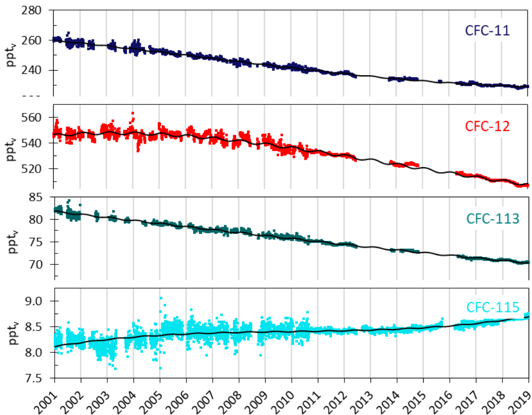
Figure 29: Daily averaged mixing ratios of the monitored CFCs at the Zeppelin observatory for the period 2001-2018: CFC-11 (dark blue), CFC-12 (red), CFC-113 (green) and CFC-115 (light blue). The solid lines are empirical fitted mixing ratios.
