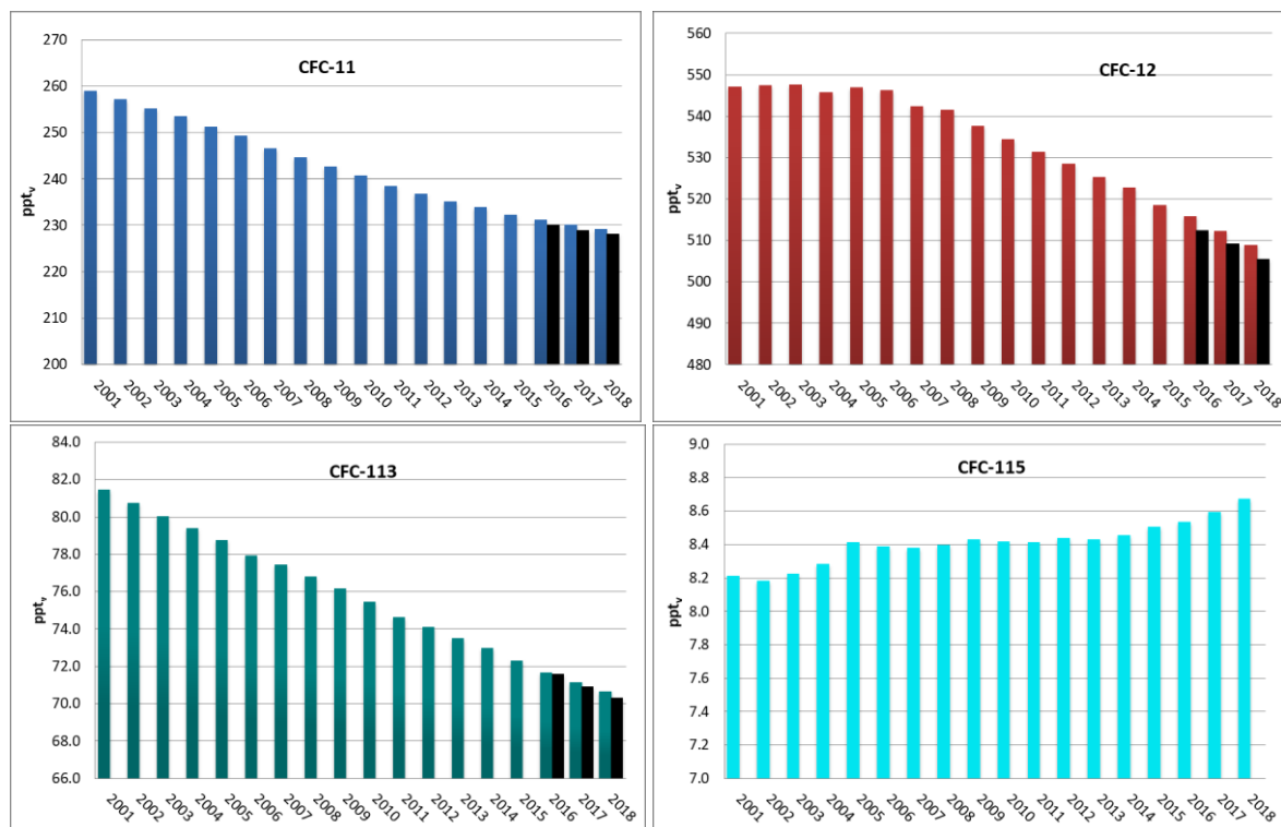
Figure 30: Development of CFC annual means at the Zeppelin Observatory for the period 2001-2018. Upper left panel: CFC-11, upper right panel: CFC-12, lower left panel: CFC-113, lower right panel: CFC-115. See Appendix I for data quality and uncertainty. The global annual means for 2016-2018 are included as black bars. All units are in ppt.
