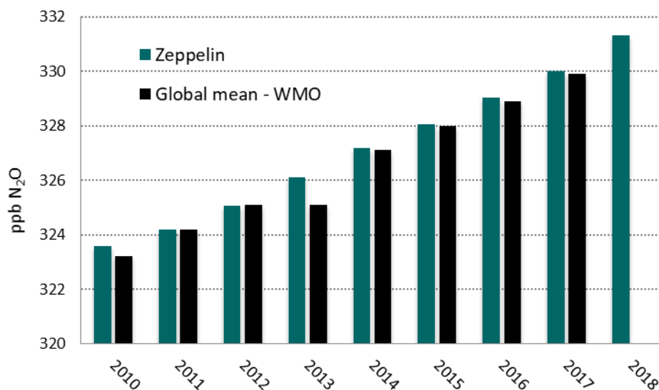
Figure 18: Annual mean concentration of N 2 O at the Zeppelin Observatory for 2010-2018.
