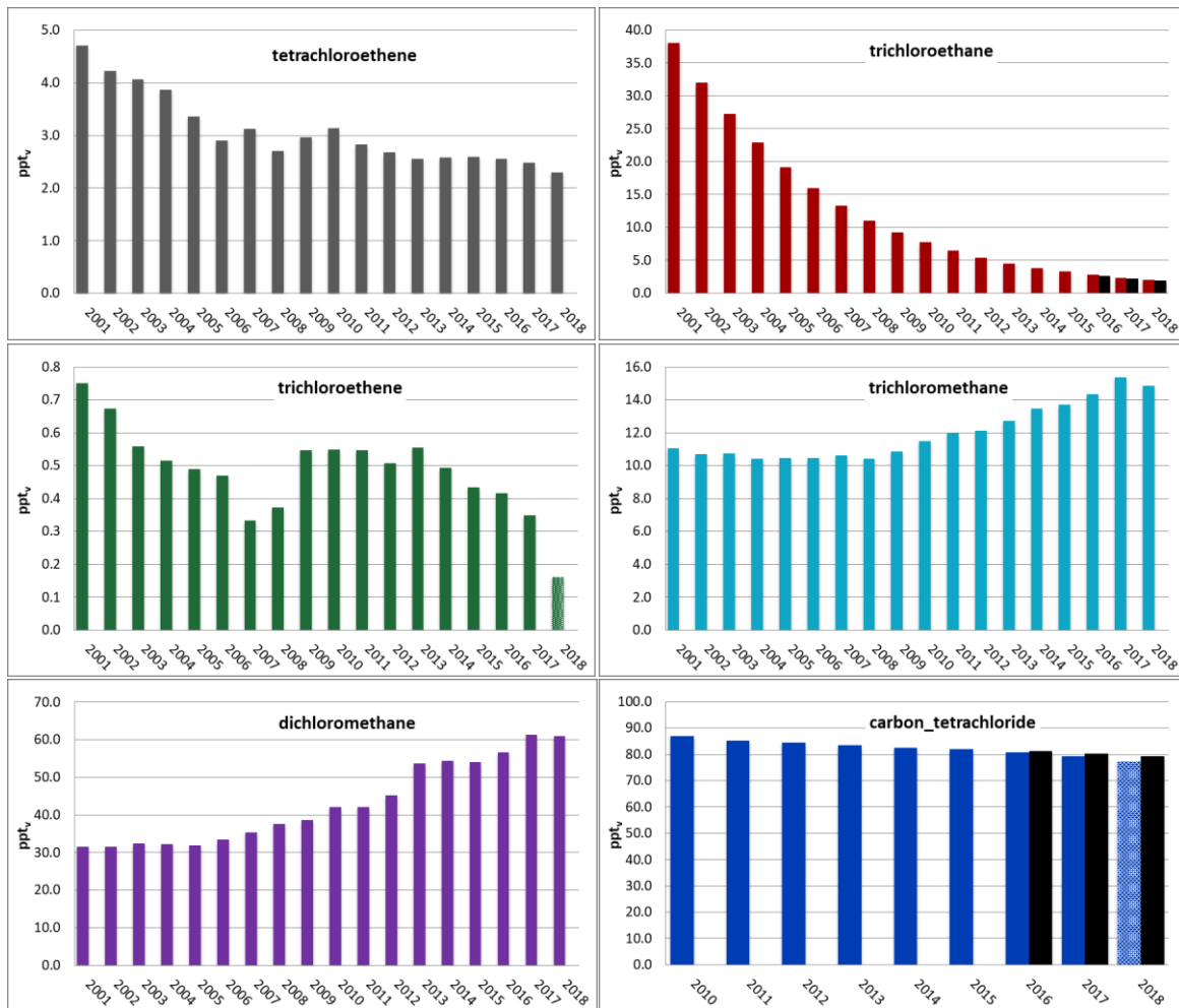
Figure 39: Annual means of the chlorinated hydrocarbons. Upper panel: tetrachloroethene (grey) and trichloroethane (red). Mid panel: trichloroethene (TCE, green) and trichloromethane (light blue). Lower panel: dichloromethane (violet) and carbon tetrachloride ( \text{CCl}_4 , dark blue). The global annual means for \text{CH}_3\text{CCl}_3 and \text{CCl}_4 in 2016-2018 are included as black bars, when available. All units are in ppt. Note that \text{CCl}_4 and TCE from 2018 are based on model data
