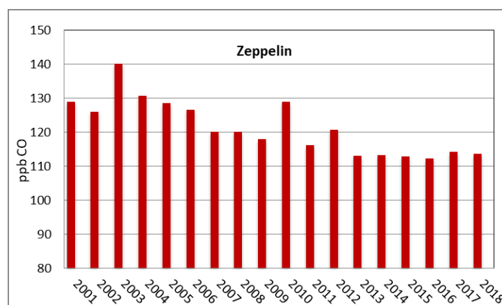
Figure 24: Development of the annual means of CO measured at the Zeppelin Observatory for the period 2001-2018. The concentrations are in ppb.
