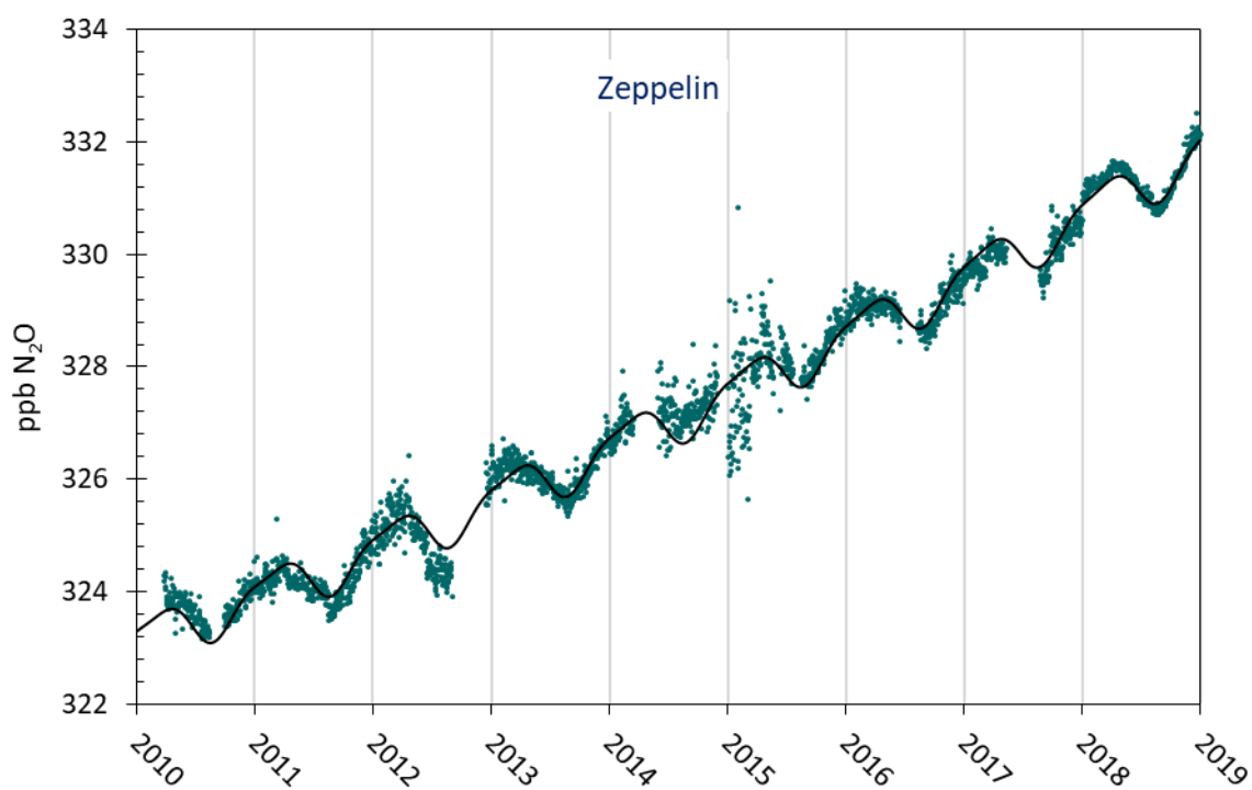
Figure 17: Measurements of N_2O at the Zeppelin Observatory for 2010-2018. The black line is empirical modelled N_2O mixing ratio.
