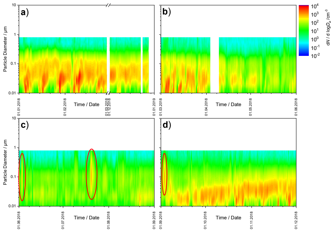
Figure 54: 2018 time series of particle number size distribution at Trollhaugen, panel a) summer, panel b) autumn, panel c) winter, panel d) spring.
