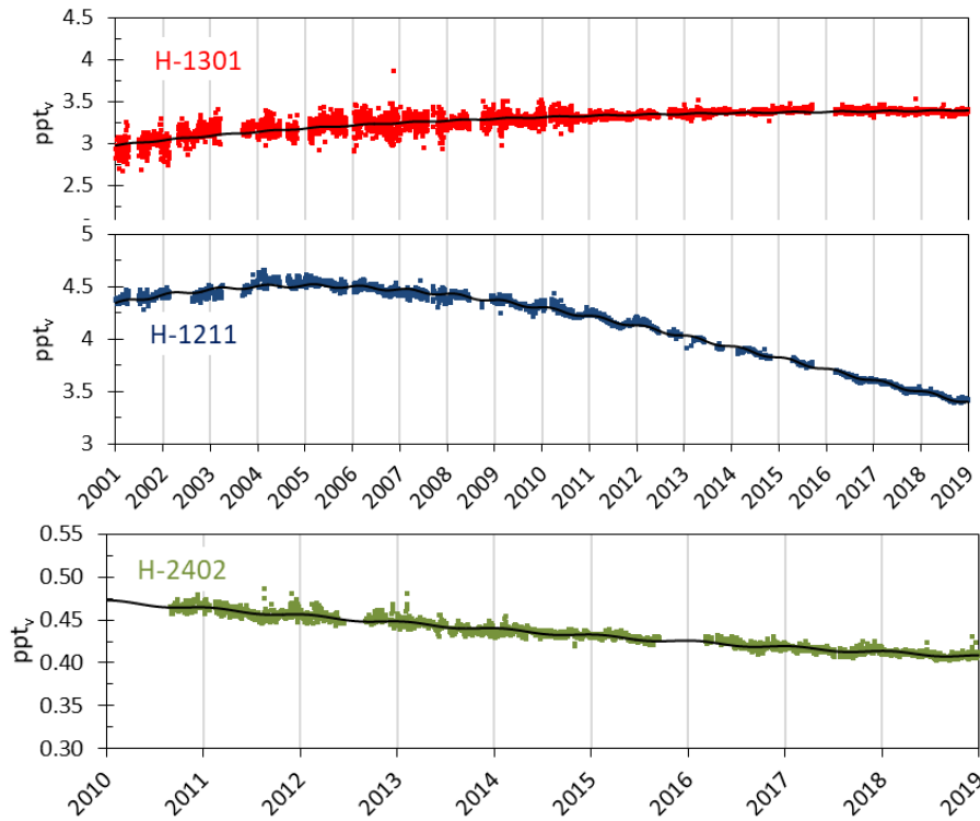
Figure 36: Daily averaged concentrations of the monitored halons at the Zeppelin Observatory. For the period 2001-2018: H-1301 (red) and H-1211 (blue). For the period 2010-2018: H-2402 (green). The solid lines are empirical fitted mixing ratios.
