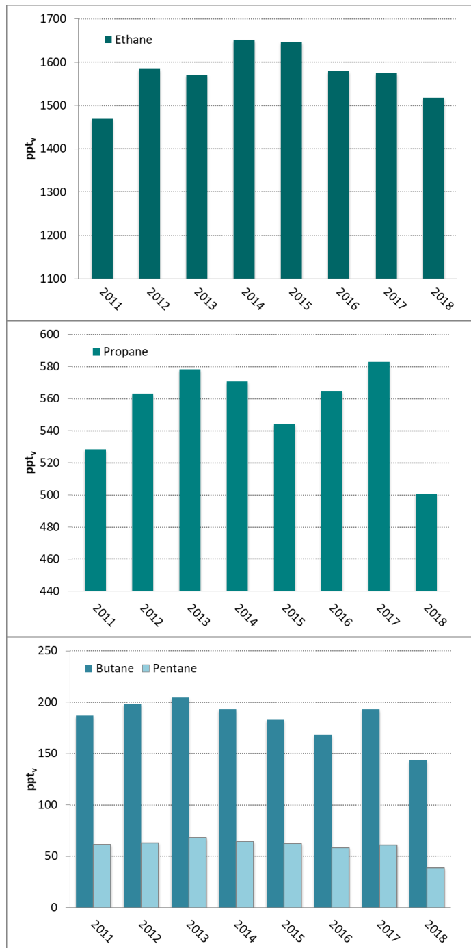
Figure 20: Development of the annual means of the measured non-methane hydrocarbons at the Zeppelin Observatory for the period 2011-2018. Upper panel in dark green: ethane, mid-panel propane, and lower panel butane and pentane. All concentrations are in ppt.
