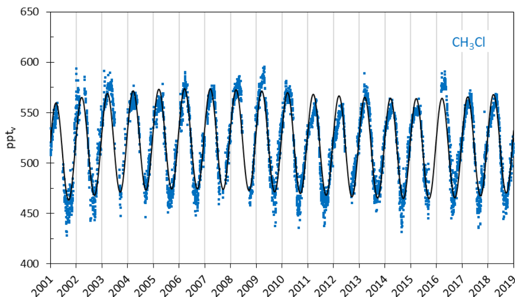
Figure 25: Observations of chloromethane, \text{CH}_3\text{Cl} , for the period 2001-2018 at the Zeppelin Observatory. Blue dots: daily averaged concentrations from the observations, solid line: empirical fitted mixing ratios.
