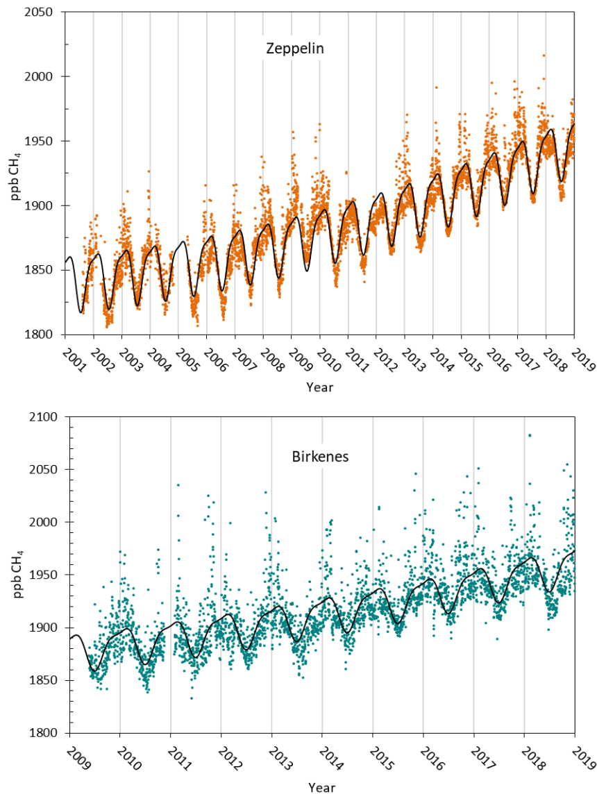
Figure 9: The upper panel shows observations of daily averaged methane mixing ratio for the period 2001-2018 at the Zeppelin Observatory. The black solid line is empirical fitted methane mixing ratio. The lower panel shows the daily mean observations for Birkenes (green dots).
