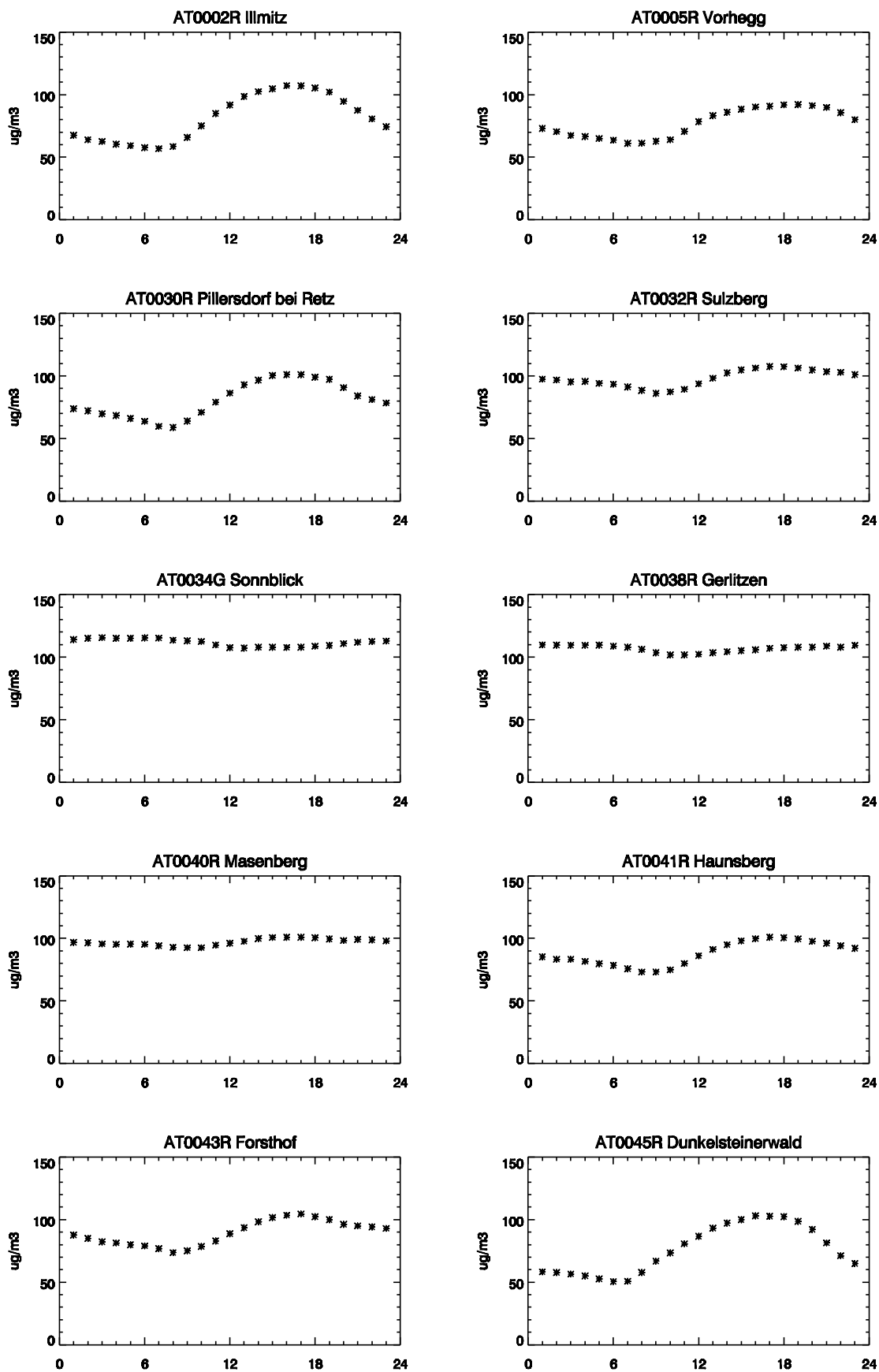
Figure 4.1: Diurnal variation, April–September 2015.
