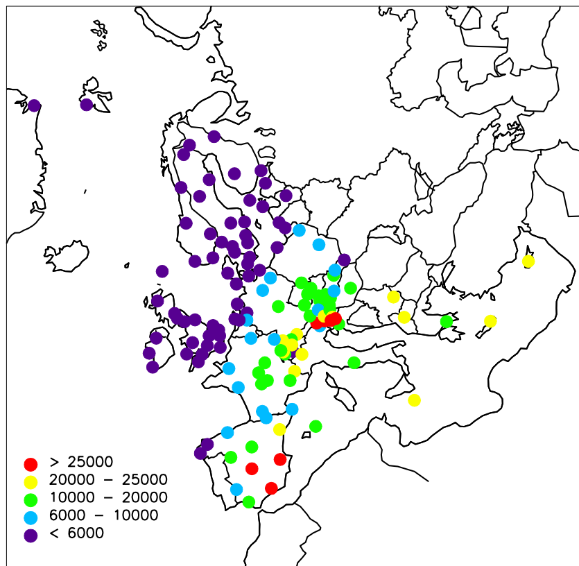
Figure 2.1: AOT40 (ppbh) April–September 2015 (daylight hours).
