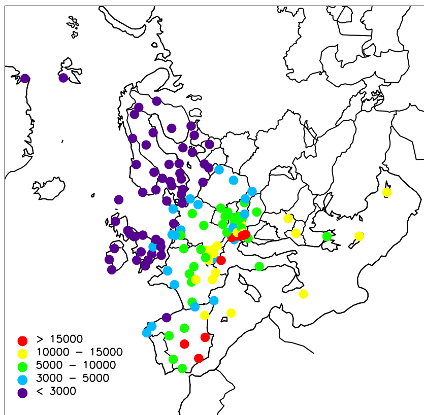
Figure 2.2: AOT40 (ppbh) May, June and July 2015 (daylight hours).
