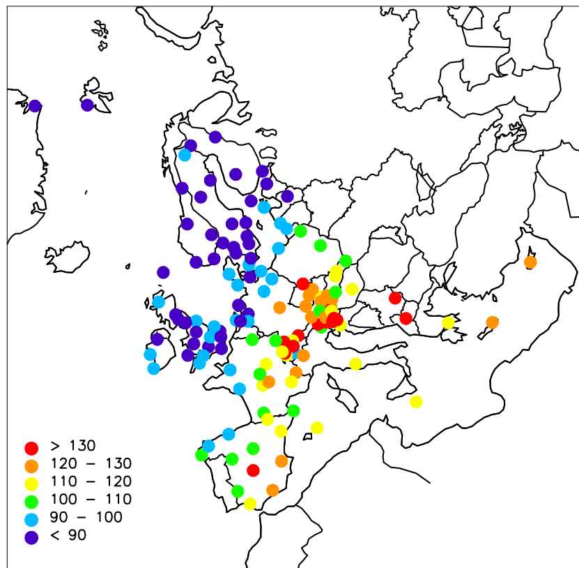
Figure 1.2: Ozone April–September 2015. 95-percentiles ( \mu\text{g}/\text{m}^3 ).
