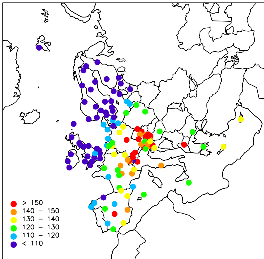
Figure 1.1: Ozone April–September 2015. 99-percentiles ( \mu\text{g}/\text{m}^3 ).
