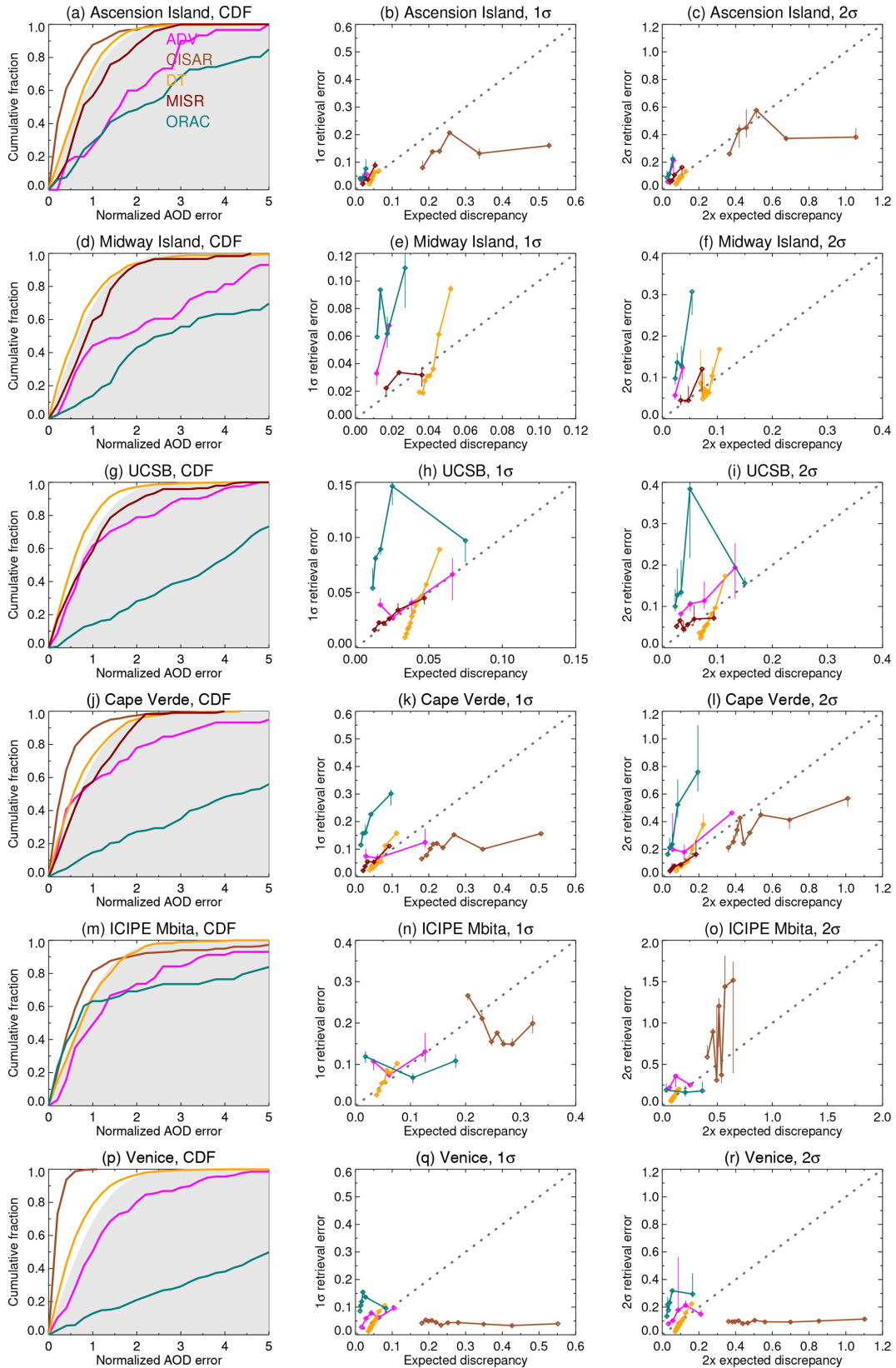
Figure 8. As Fig. 7, except for AERONET sites used for over-water retrieval evaluation.
