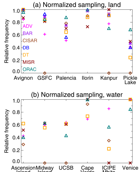
Figure 6. Site-to-site corrected sampling \hat{n} for each data set, shown on a relative scale. Symbols are used to aid in differentiating overlapping data points but carry no further information.
