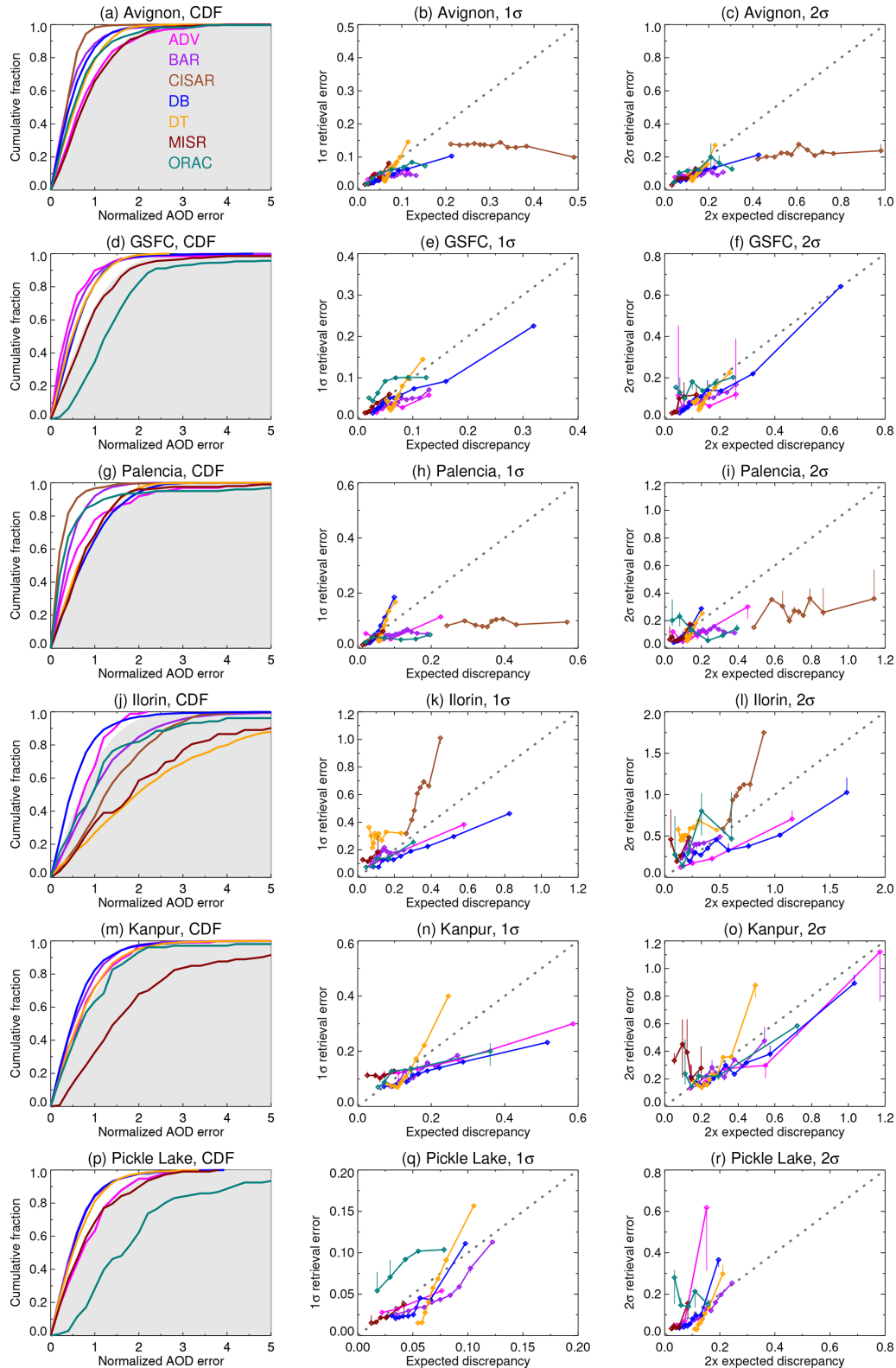
Figure 7. Evaluation of pixel-level uncertainty estimates for overland retrievals. Each row corresponds to a different AERONET site, and colours are used to distinguish data sets. The left-hand column shows a CDF of the absolute normalized retrieval error |\Delta_N| (see Fig. 3b), and the middle and right columns show 1\sigma and 2\sigma expected discrepancy ED vs. absolute retrieval errors |\Delta_S| (see Fig. 4), respectively. In the left column, theoretical expectations are shaded grey; in the others, the 1:1 line is indicated dashed in grey, and vertical bars indicate the uncertainty on the bin value, as described in the text.
