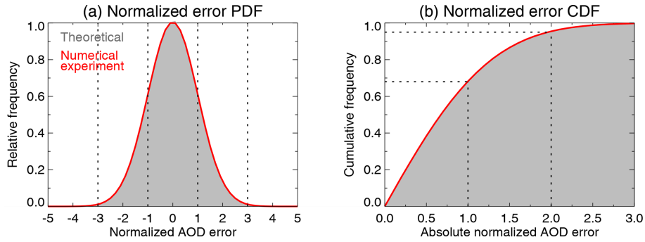
Figure 3. (a) PDF and (b) CDF of normalized error distributions drawn from the numerical simulations in Fig. 1; theoretical (grey shading) and simulation (red) results lie on top of one another. Note that the CDF is of absolute normalized error. Dashed lines indicate various well-known percentage points of Gaussian distributions.
