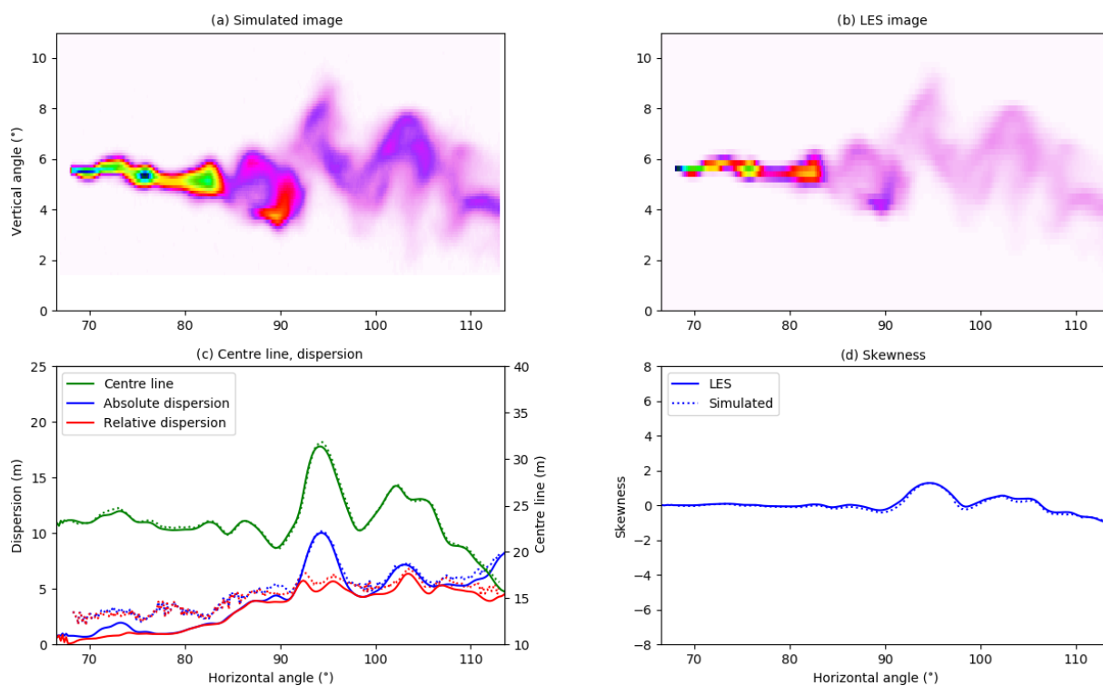
Figure 4. (a) The plume apparent absorbance for camera A from Fig. 3c. (b) The LES column density integrated along the line of sight. Colour scales in (a) and (b) are relative and thus no colour bars are provided. (c) The centre line, absolute, and relative dispersions. (d) The skewness.
