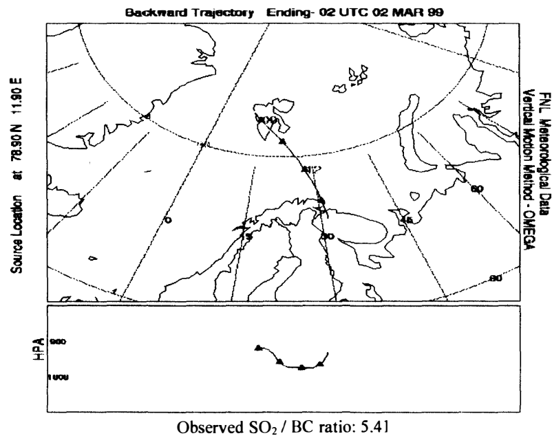
Fig. 3. Examples of airmass back trajectories associated with high BC concentrations at Ny-Ålesund, coinciding with the two main air pollution sources for the High Arctic, the industrial complexes at Norilsk and Kola peninsula of Russia. Back trajectories performed by means of the NOAA Hysplit model through their network service.
