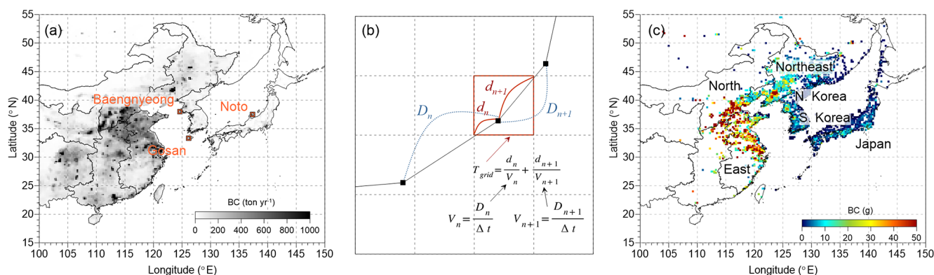
Figure 1. (a) The location of the three measurement sites (Baengnyeong, Gosan, and Noto) and the black carbon (BC) emission rate ( \text{tyr}^{-1} ) over East Asia from the Regional Emission inventory in ASia (REAS) version 2.1 (Kurokawa et al., 2013). (b) Illustration of residence time calculated based on the HYSPLIT backward trajectory that passed over a single grid cell (see details in the text). (c) The location of administrative districts, and the spatial distribution of the mean BC mass in the potential emission region, which is the highest BC mass grid of each trajectory. The BC mass was obtained by multiplying (a) the emission rates and (b) the residence time.
