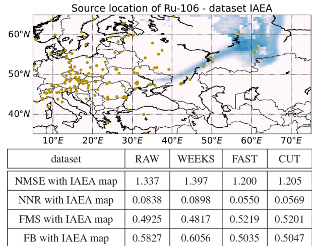
Figure 10. Top: source location of the release of ^{106}\text{Ru} via marginal log likelihood, using the IAEA dataset. Bottom: the computed normalized mean square error (NMSE), the normalized mean square error of the distribution of the normalized ratios (NNR), the figure of merit in space (FMS), and the fractional bias (FB) between the source location results obtained using the IAEA dataset and the RAW, WEEKS, FAST, and CUT datasets.
