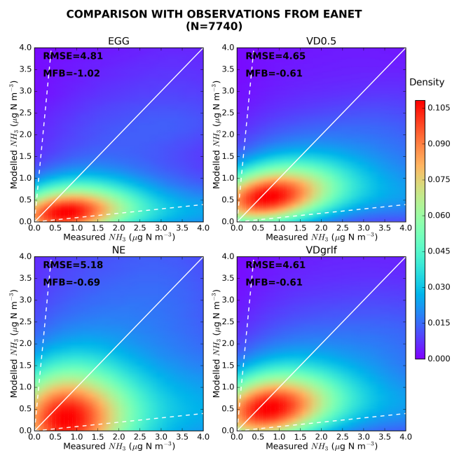
Figure 7. Validation of modelled concentrations of ammonia for different emissions datasets (EGG, VD0.5, NE and VDgrlf) against ground-based measurements from EANET for the 10-year (2008–2017) study period. Scatterplots of modelled against measured concentrations for the aforementioned emission inventories were plotted with the Kernel density estimation, which is a way to estimate the probability density function (PDF) of a random variable in a non-parametric way.
