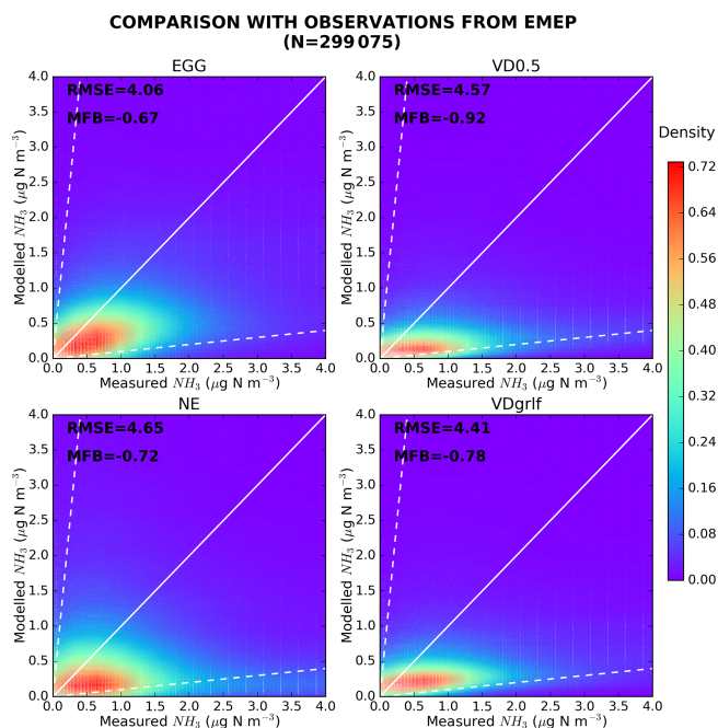
Figure 5. Validation of modelled concentrations of ammonia for different emissions datasets (EGG, VD0.5, NE and VDgrlf) against ground-based measurements from EMEP for the 10-year (2008–2017) study period. Scatterplots of modelled against measured concentrations for the aforementioned emission inventories were plotted with the Kernel density estimation, which is a way to estimate the probability density function (PDF) of a random variable in a non-parametric way.
