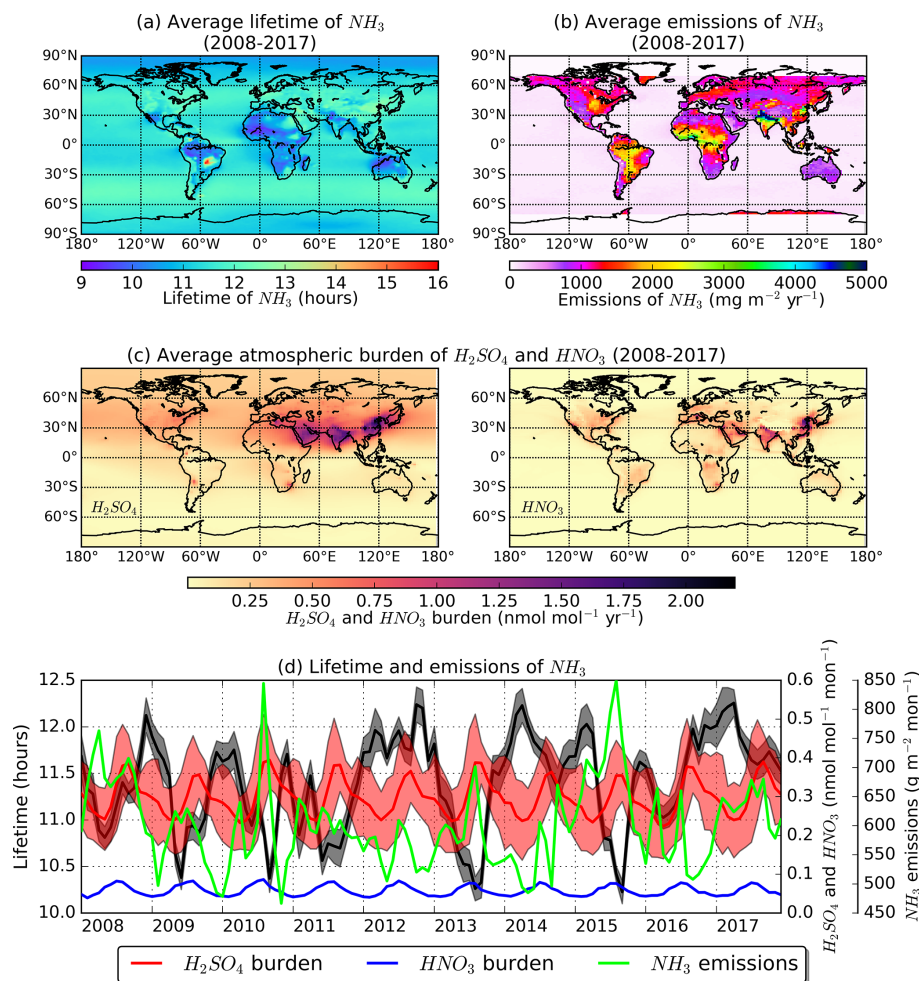
Figure 1. (a) The 10-year average model lifetime of ammonia calculated from LMDz-OR-INCA; (b) total annual emissions averaged over the 10-year period (NE emissions); (c) atmospheric burden of the reactants sulfuric acid and nitric acid calculated in the model; and (d) monthly time series of lifetime (black), ammonia emissions (green), sulfuric (red) and nitric acid column concentrations (blue) for the whole 10-year period.
