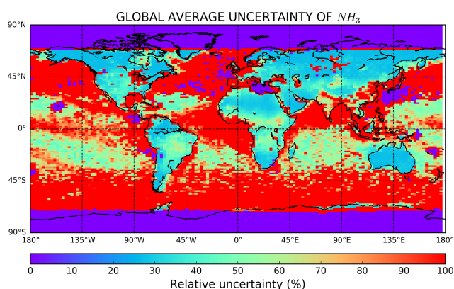
Figure 10. The 10-year average relative uncertainty of modelled surface concentrations expressed as the standard deviation of surface concentrations from a model ensemble (Table 1) divided by the average.
