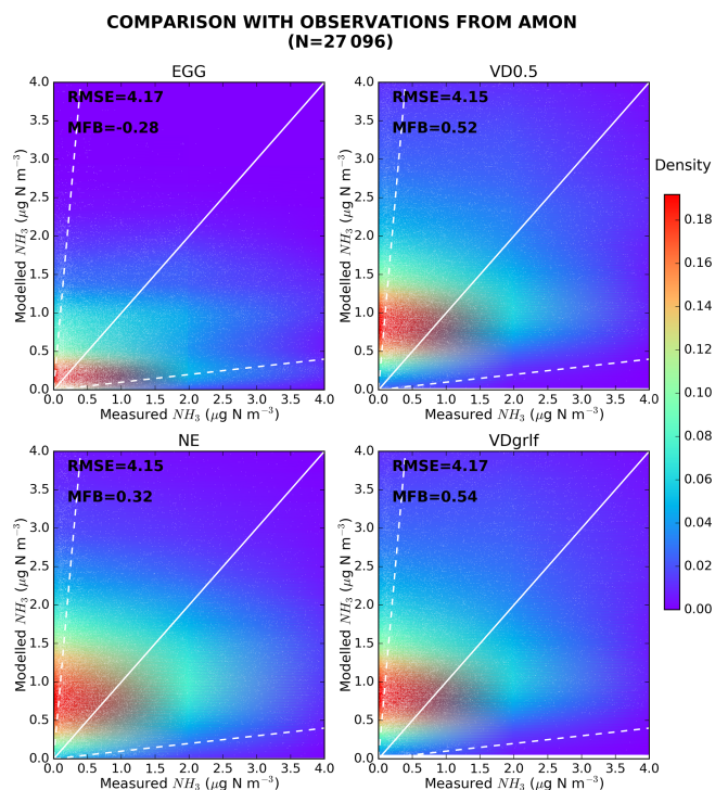
Figure 6. Validation of modelled concentrations of ammonia for different emissions datasets (EGG, VD0.5, NE and VDgrlf) against ground-based measurements from AMON for the 10-year (2008–2017) study period. Scatterplots of modelled against measured concentrations for the aforementioned emission inventories were plotted with the Kernel density estimation, which is a way to estimate the probability density function (PDF) of a random variable in a non-parametric way.
