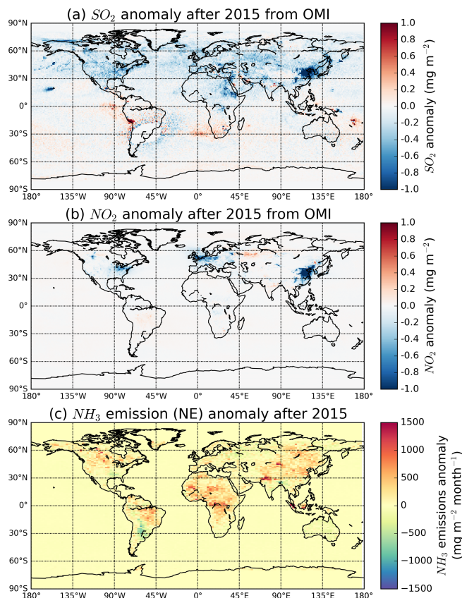
Figure 2. Annual average total column (a) sulfur dioxide and (b) nitrogen dioxide anomaly after 2015 from OMI and (c) annual average emission anomaly of ammonia calculated from IASI in the present study (NE).
