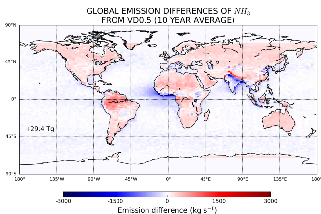
Figure 3. Global differences of ammonia emissions calculated in the present study (NE) from those calculated using Van Damme et al. (2018) gridded concentrations applying a constant lifetime of 0.5 d (VD0.5). The results are given as 10-year average (2008–2017), and the number denotes the annual difference in the emissions.
