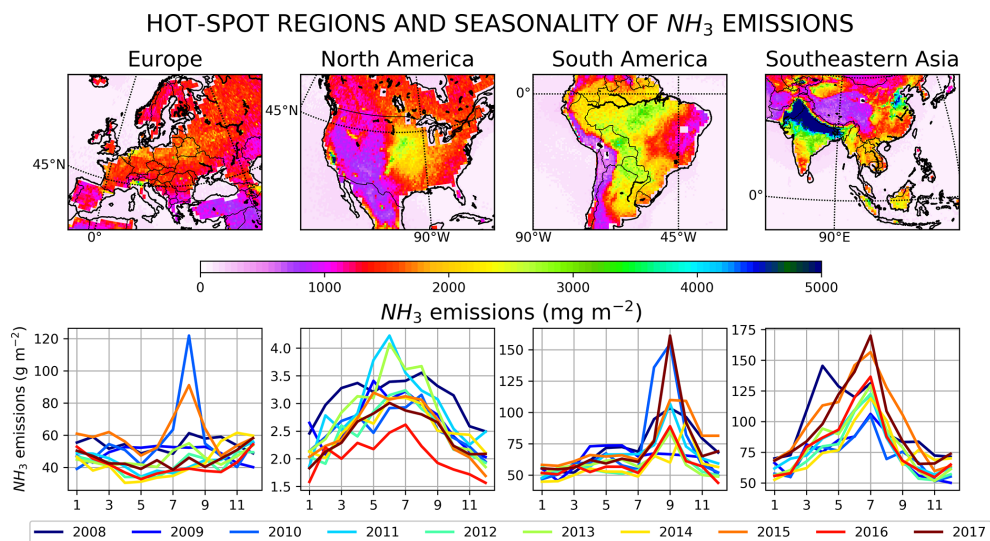
Figure 4. Total annual emissions of ammonia averaged over the 10-year period (2008–2017) in Europe, North America and South America, and Southeastern Asia, which are regions characterized by the largest contribution to the global ammonia budget. In the bottom panels the monthly variation of the emissions is shown for each year of the study periods.
