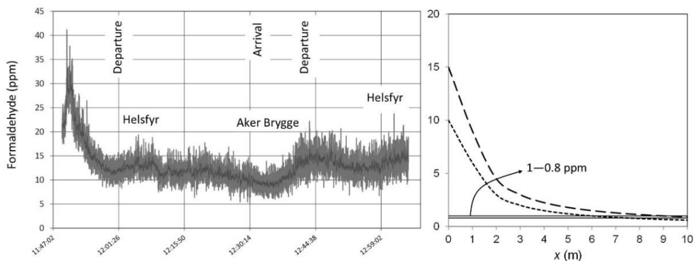
Fig. 1: Formaldehyde measured from the exhaust pipe of an E95 bus during on-road driving conditions (left) and estimated along the center line of the dispersion plume as a function of distance from the exhaust pipe (right).
