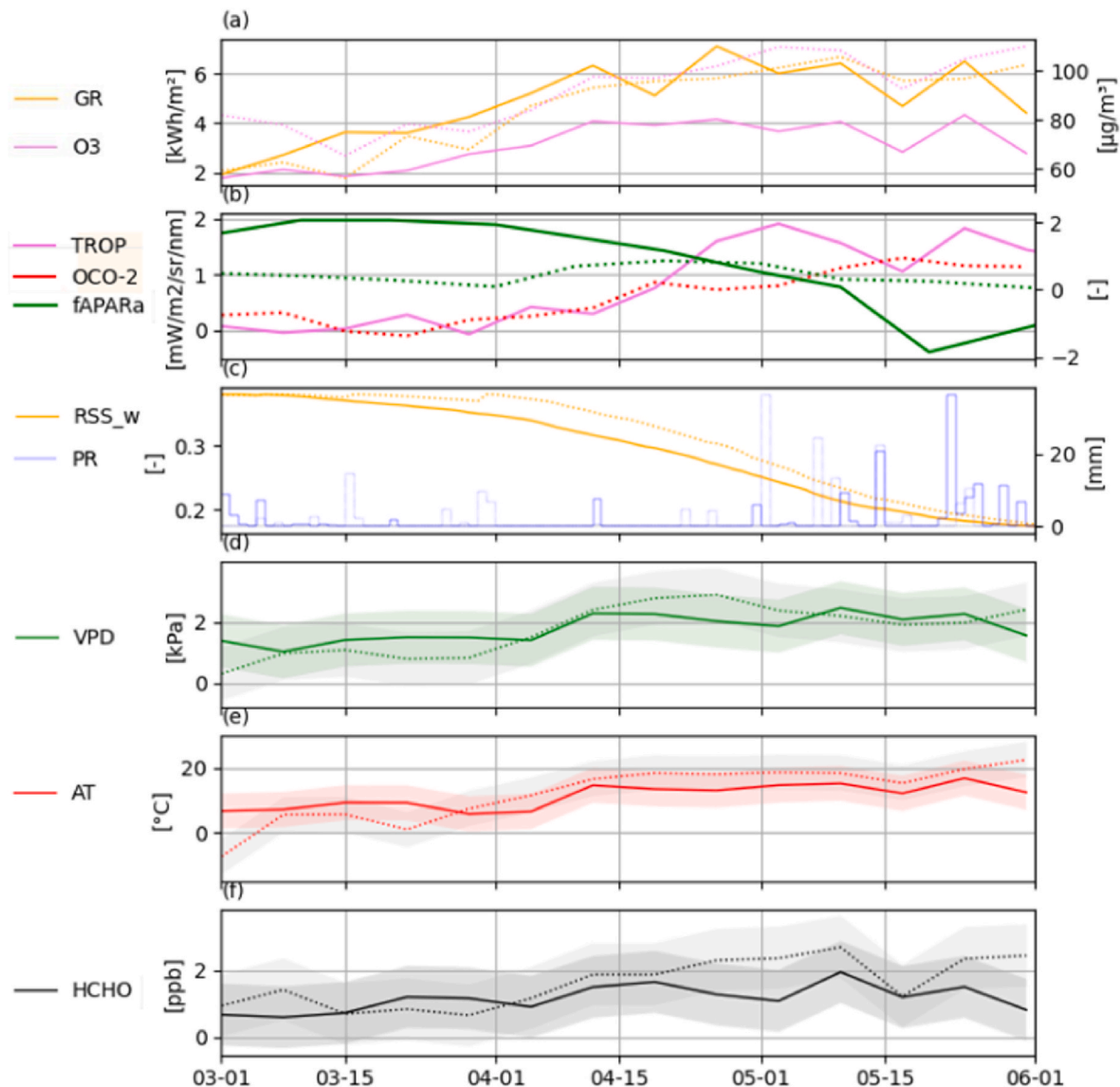
Fig. 3. Time series of weekly (a) \text{O}_3 (pink) and GR (orange), (b) SIF (TROPOMI: pink, \text{OCO}_2 : red), fAPARa (green) (c) \text{RSS}_w (orange), PR (blue), (d) VPD (green) (e) AT (red), (f) HCHO (black) comparing MAM20 (solid lines) to MAM18 (dotted lines). The shading in (d)–(f) shows the standard deviation of daily values.
