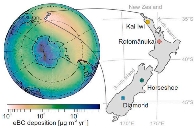
Fig. 1. Map of Southern Hemisphere and study region showing FLEXPART atmospheric aerosol deposition fluxes obtained from a forward simulation (Stohl et al., 2005; Pisso et al., 2019) for equivalent black carbon (eBC) emissions from New Zealand. Selected charcoal sites are shown for comparison (Gray circles; DL = Dove Lake; GP = Granta Pool; BRL = Big Reedy Lagoon; SL = Swallow Lagoon). Right panel shows zoom of New Zealand with location of the four lake sites across the South and North Island.
