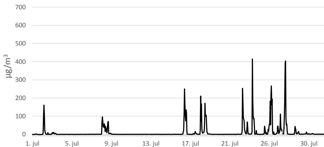
SO 2 - Svanvik august 2015
