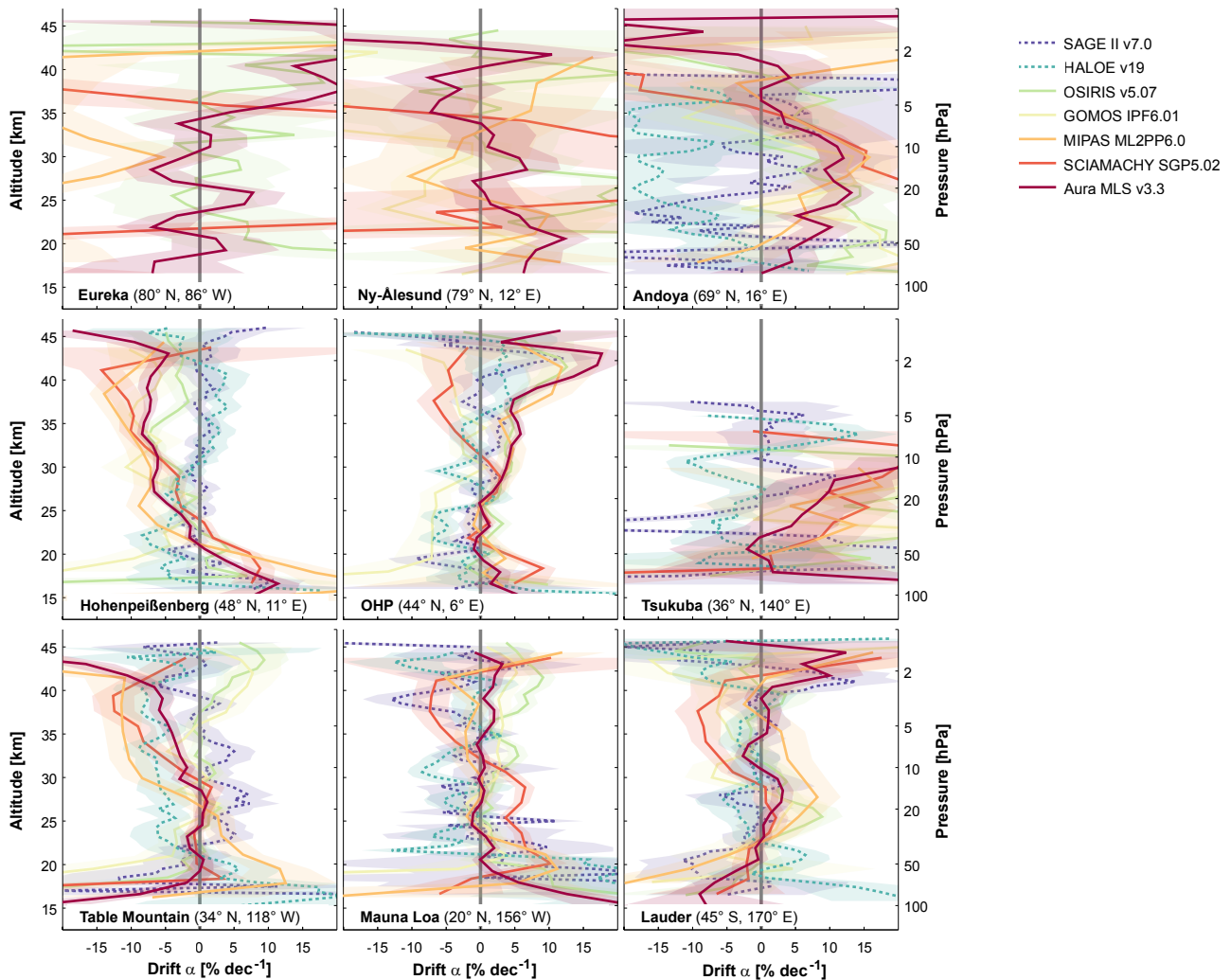
Figure 4. Comparison of the vertical structure of the drift \alpha of two historic (dashed lines) and five recent (solid) satellite records relative to stratospheric lidar observations at nine NDACC stations. The shaded area represents the unadjusted 68 % confidence interval, which does not include possible uncertainties from differences in sampling or from inhomogeneities in the lidar network. The analysis is performed in the native profile representation of each satellite record.
