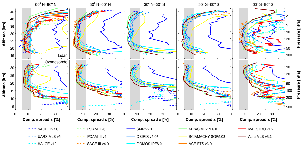
Figure 11. Similar as Fig. 10, but for the comparison spread s . The spread is mostly between 5 and 12 % (grey shaded area) in the middle and upper stratosphere.
