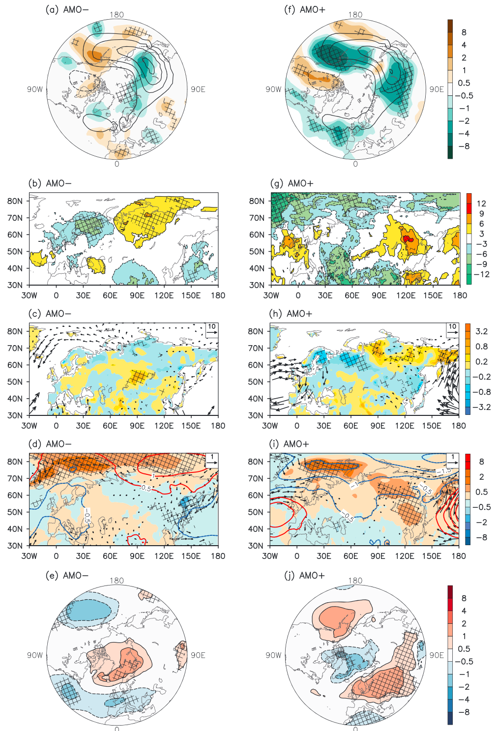
Figure 4. As in Figure 3, except for ERA20CM (1979/1980–2009/2010), using a different color scale. Those values exceeding 90% confidence interval are denoted by slash.
