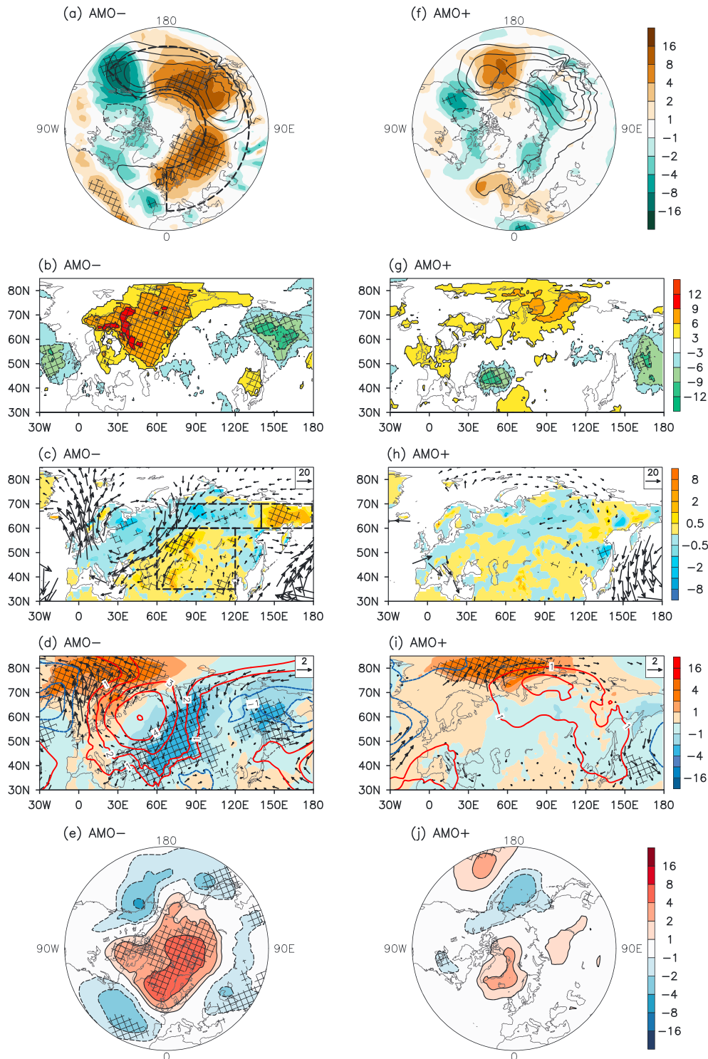
Figure 3. (a) The climatology (contours; interval: 10^{-2} \text{ m}^2 \text{ s}^{-2} ) and regression (shaded; unit: 10^{-3} \text{ m}^2 \text{ s}^{-2} ) upon the negative Atlantic Arctic sea ice cover (AASIC) index for the cold Atlantic Multidecadal Oscillation (AMO-) period of December 150 hPa F_Z . The regression upon the negative AASIC index for the AMO- period of (b) the frequency of blocking heights (unit: %), (c) Eurasian snow depth (shaded; unit: cm) and integrated water vapor transport (vectors; unit: \text{kg m}^{-1} \text{ s}^{-1} ), (d) sea level pressure (SLP) (contours; unit: hPa)/horizontal winds at 10 m (vectors; unit: \text{m s}^{-1} )/surface air temperature (shaded; unit: ^{\circ}\text{C} ) in December, and (e) SLP (unit: hPa) in February. Those values exceeding 95% confidence interval are denoted by slash. (f–j) As in Figures 3a–3e, except for the AMO+ period. The data sets are derived from ERA-I (1979/1980–2016/2017) and ERA-I/Land (1980–2014). The black frames in Figures 3a and 3c depict the regions used to define F_Z and ESD indices, respectively (see supporting information S1).
