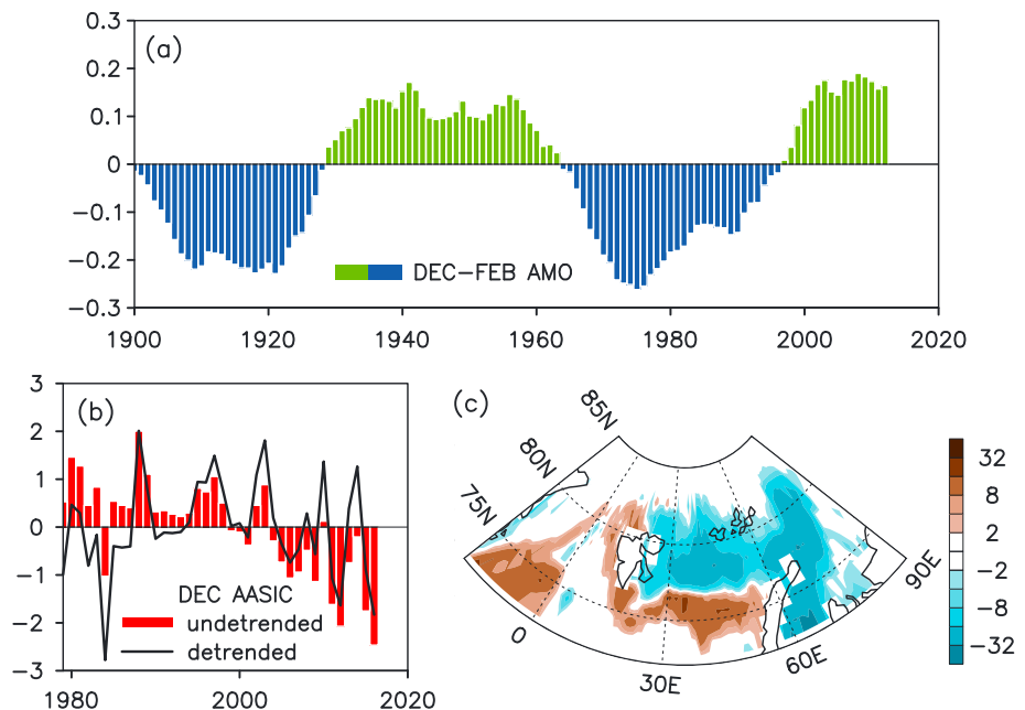
Figure 1. (a) Time evolution of the smoothed December–February mean Atlantic Multidecadal Oscillation (AMO) index for 1900/1901–2011/2012. (b) Time evolution of the undetrended (red bar) and detrended (black line) December Atlantic Arctic sea ice cover (AASIC) index for 1979–2016. (c) The decadal difference of the standard deviation (unit: %) of December sea ice concentration between 1979–1995 and 1996–2016 (1979–1995 minus 1996–2016).
