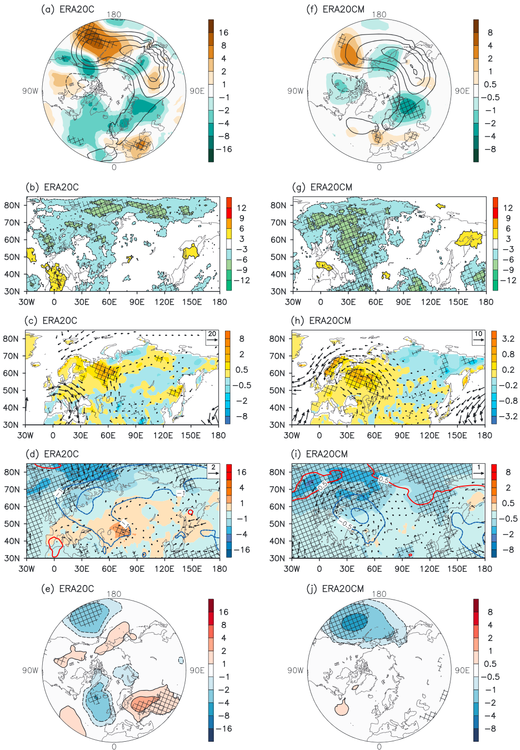
Figure 2. (a) The climatology (contours; interval: 10^{-2} \text{ m}^2 \text{ s}^{-2} ) and composite difference (shaded; unit: 10^{-3} \text{ m}^2 \text{ s}^{-2} ) between the cold and warm phases of the Atlantic Multidecadal Oscillation (AMO– minus AMO+) of December 150 hPa Fz. The composite difference between the AMO– and AMO+ of (b) the frequency of blocking heights (unit: %), (c) Eurasian snow depth (shaded; unit: cm) and integrated water vapor transport (vectors; unit: \text{kg m}^{-1} \text{ s}^{-1} ), (d) sea level pressure (SLP) (contours; unit: hPa)/horizontal winds at 10 m (vectors; unit: \text{m s}^{-1} )/surface air temperature (shaded; unit: °C) in December, and (e) SLP (unit: hPa) in February. Those values exceeding 95% confidence interval are denoted by slash. The data sets are derived from ERA20C (1900/1901–2009/2010). (f–j) As in Figures 2a–2e, except for ERA20CM (1900/1901–2009/2010), using a different color scale.
