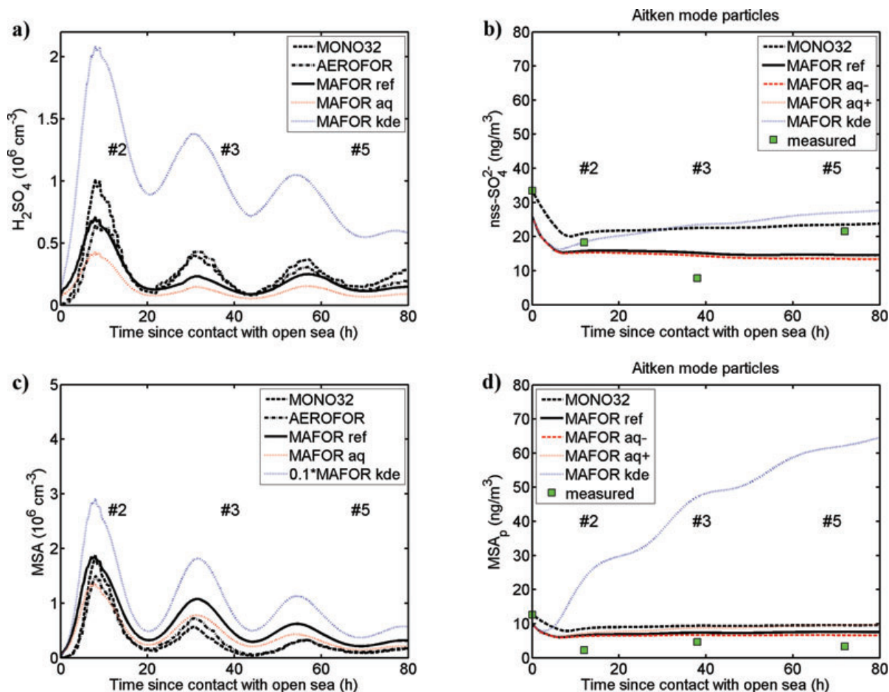
Fig. 5. Concentration time series of gas-phase and particulate phase sulphuric constituents in the marine transport scenario: (a) gaseous H_2SO_4 , (b) particulate nss-SO_4^{2-} in Aitken mode, (c) gaseous MSA and (d) particulate MSA_p in Aitken mode. Simulation with MONO32 (dashed black), with AEROFOR (dash-dotted black, only gas-phase constituents), with MAFOR using the reference (ref) configuration (dashed black), with MAFOR (aq) allowing for partitioning to the aqueous phase (red lines), and with MAFOR (kde; dotted blue lines) using the rate constant of CH_3SO_2 thermal decomposition given by Kerminen and Leck (2001). Observed nss-SO_4^{2-} and MSA_p concentrations in the Aitken mode aerosol obtained during AOE-96 are indicated as green squares. Note that for MAFOR (kde) gaseous MSA concentrations were scaled by a factor of 0.1. For details on the uncertainty tests see text.
