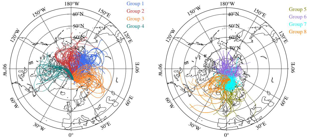
Fig. 2. Cluster allocation of ensemble trajectories at all heights (850, 700 and 500 hPa) for Ny-Ålesund 1995–2008.
