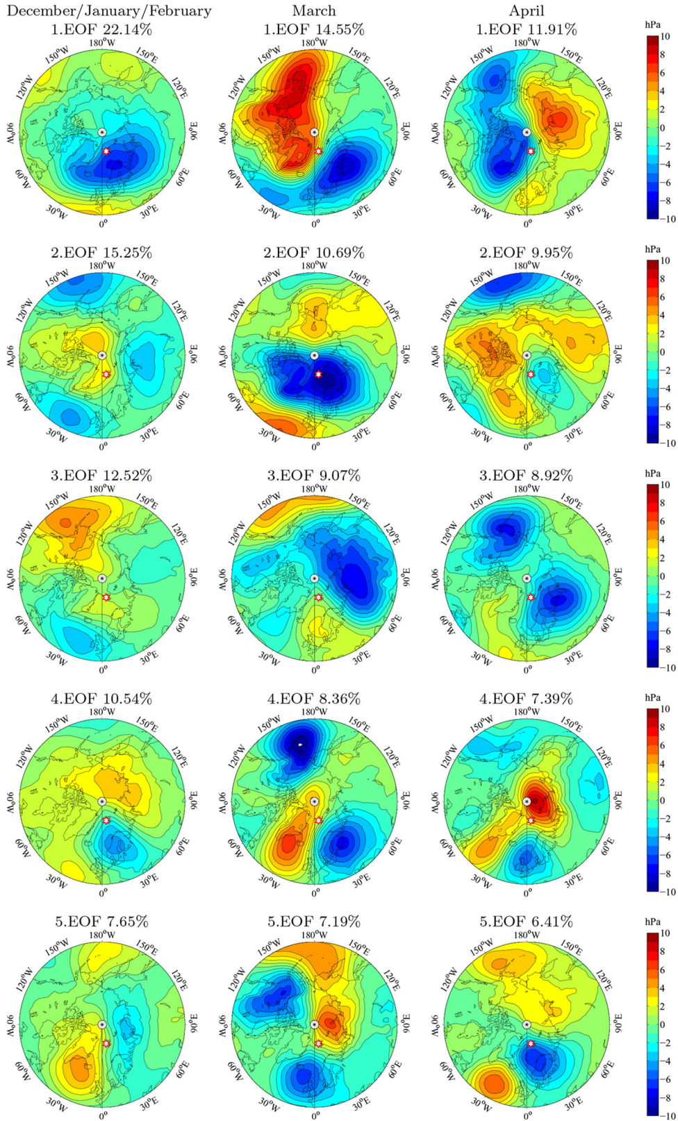
Fig. 10. First five EOF of mean sea-level pressure of three periods: left – December, January and February (1995–2008); middle – March (1995–2008); right – April (1995–2008) and their variance in %. The white star marks the position of Ny-Ålesund, respectively Spitsbergen.
