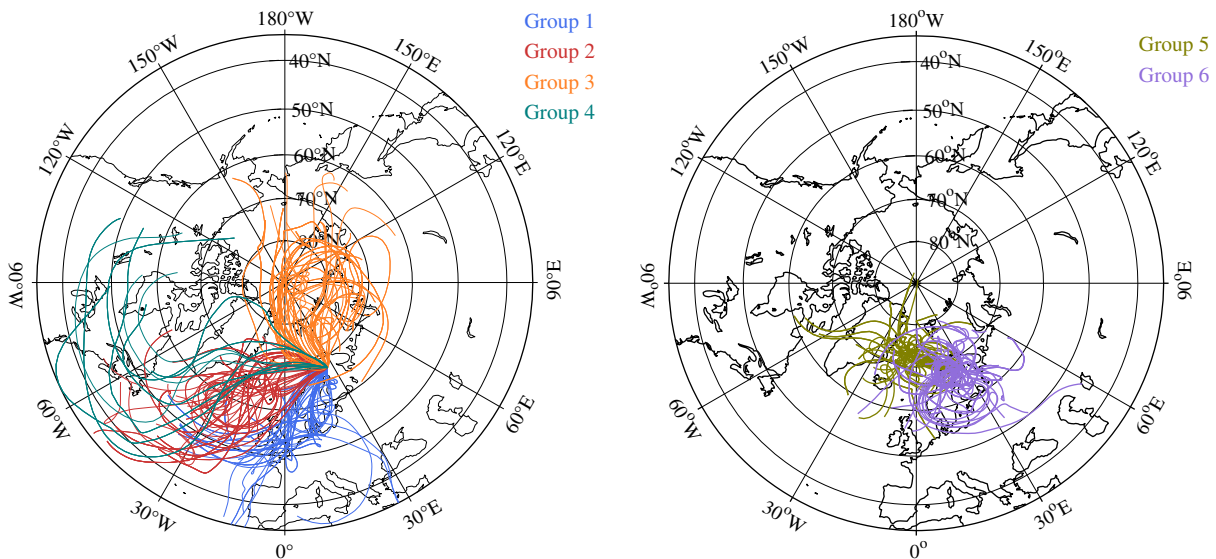
Fig. 4. Cluster allocation of ensemble trajectories at all heights (850, 700 and 500 hPa) for Sodankylä 2004–2007.
