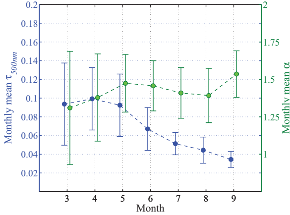
Fig. 7. Monthly means of \tau_{500nm} and \alpha in Ny-Ålesund.
