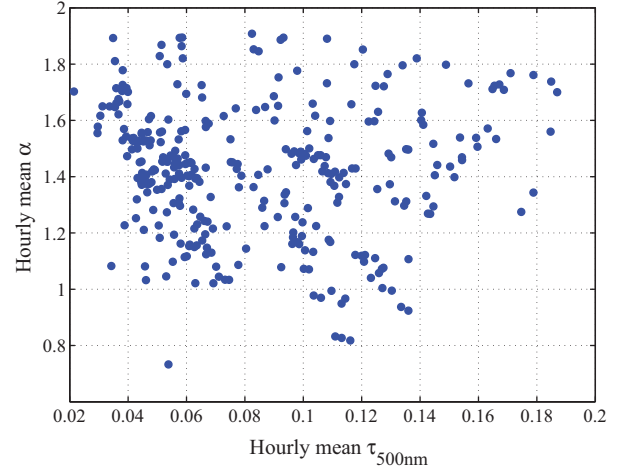
Fig. 11. Scatter plot of all hourly mean \tau_{500\text{nm}} and \alpha measured in Ny-Ålesund 1995–2008 and assigned to a trajectory cluster.
