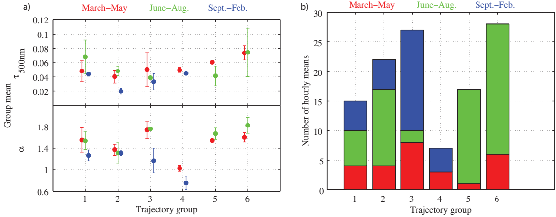
Fig. 5. (a) Mean values and standard deviation of \tau_{500\text{nm}} and \alpha and (b) number of hourly mean AOD in different trajectory groups from Sodankylä 2004–2007. Seasonal separation: spring – red; summer – green; autumn – blue.
