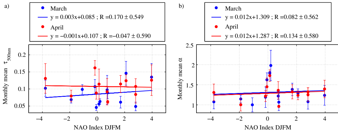
Fig. 9. Correlation between NAO-Index and monthly mean AOD in March (blue) and April (red) for Ny-Ålesund 1995–2008. Drawn are the monthly mean standard deviation and the linear regression of a) \tau_{500\text{nm}} and b) \alpha . The parameters of the regression, including the correlation coefficient and their confidence range, are shown in the legend.
