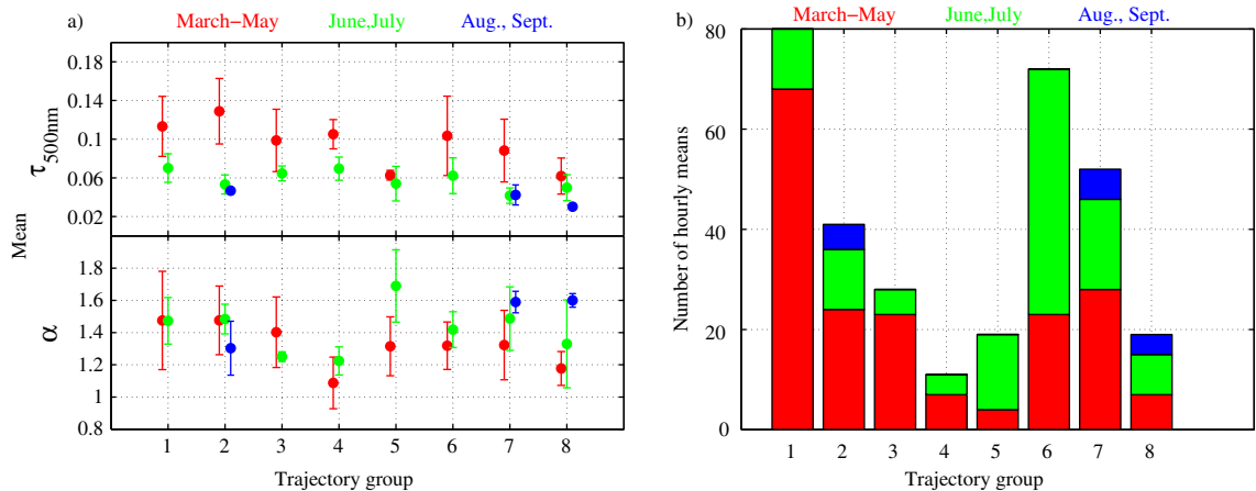
Fig. 3. (a) Mean values and standard deviation of \tau_{500\text{nm}} and \alpha and (b) number of hourly mean AOD in different trajectory groups from Ny-Ålesund 1995–2008. Seasonal separation: spring – red; summer – green; autumn – blue.
