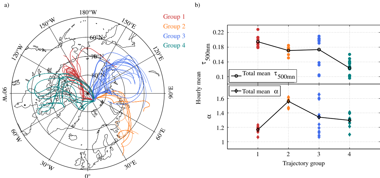
Fig. 6. (a) Clustering of the ensemble trajectories at all heights (850, 700, 500 hPa) from NP-35 between 14 March and 7 April, 2008, and (b) hourly mean of \tau_{500\text{nm}} and \alpha in the different trajectory groups and the group mean of \tau_{500\text{nm}} and \alpha .
