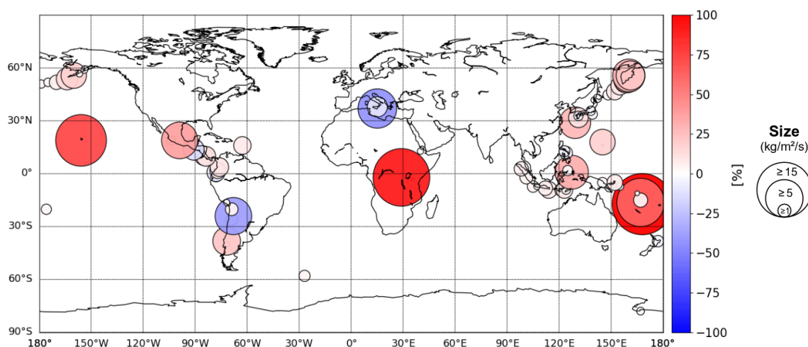
Figure 2. The 2013 annual average ratio between volcanic \text{SO}_2 emissions in the Carn et al. (2016, 2017) and Andres and Kasgnoc (1998) inventories. The size of the circles represents the absolute difference in kilograms per meter per second ( \text{kg m}^{-2} \text{s}^{-1} ), while the color represents the relative difference in percent.
